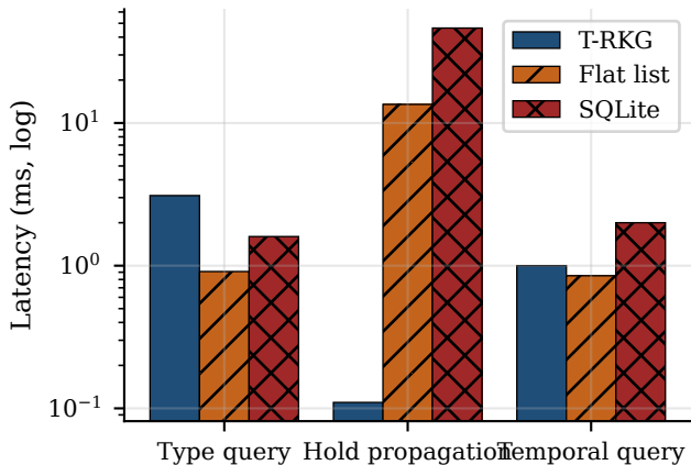
Performance vs. flat / relational baselines (10K records)
