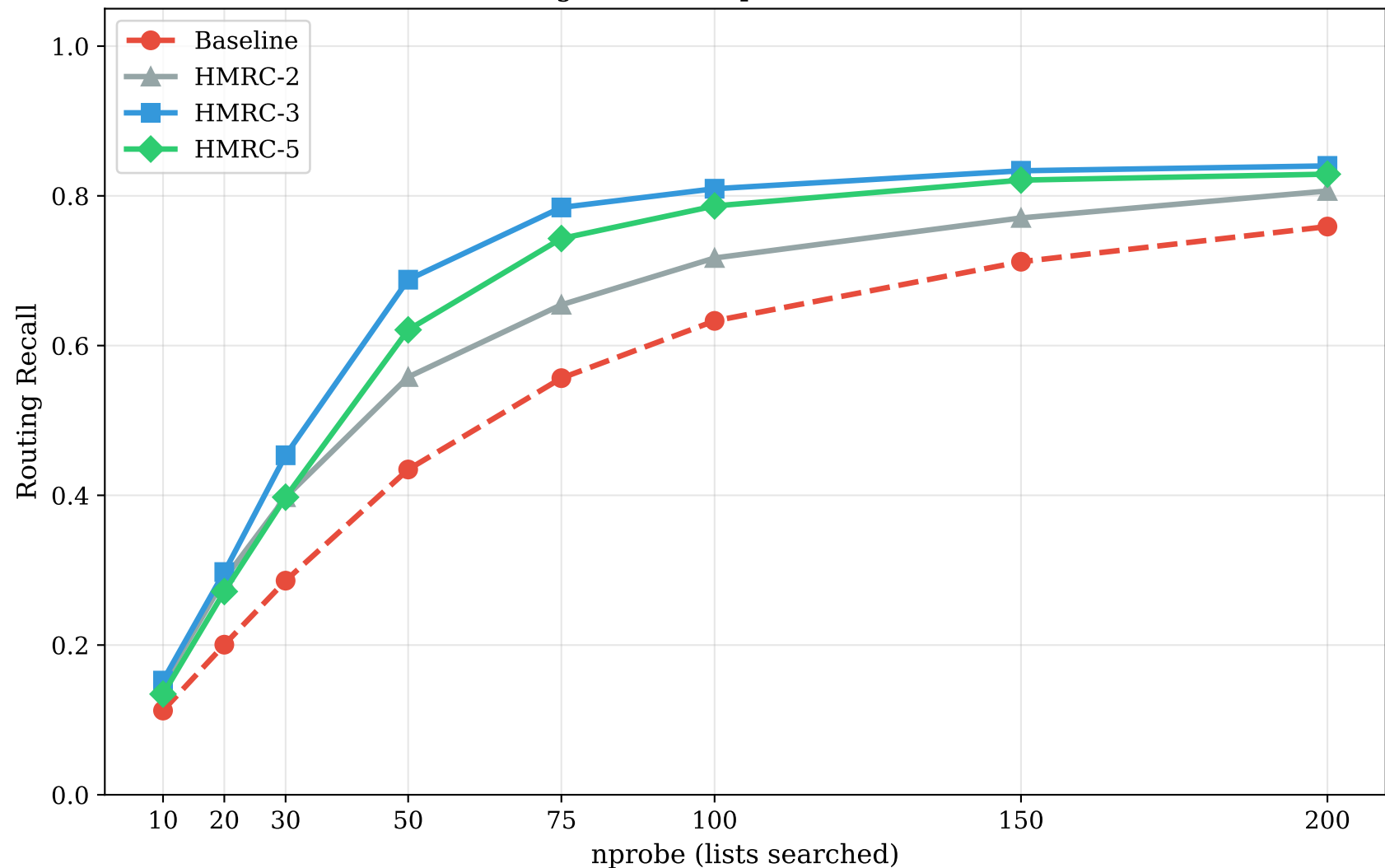
FAISS IVF: Routing Recall vs nprobe (MSMARCO-1M, Semi-3)
