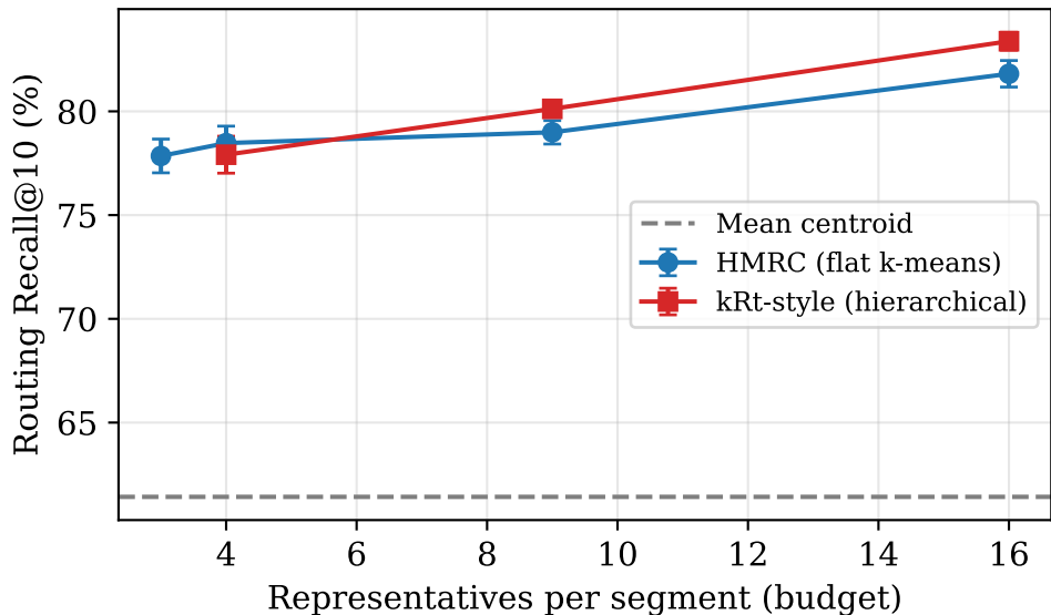
MSMARCO-100K: flat vs hierarchical reps. (semi-structured segments, 5 seeds, 95% CI)
