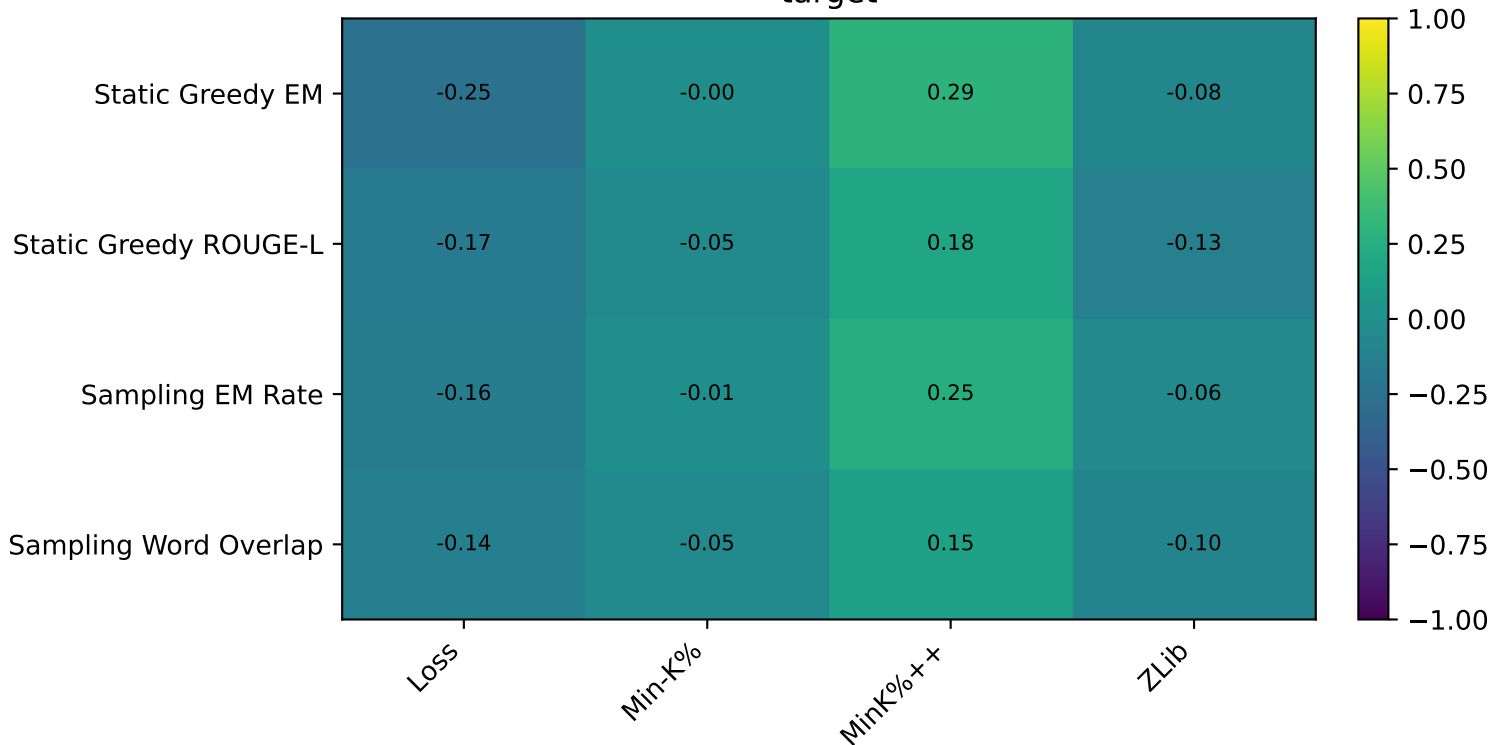
Mean within-cell Kendall \tau target
