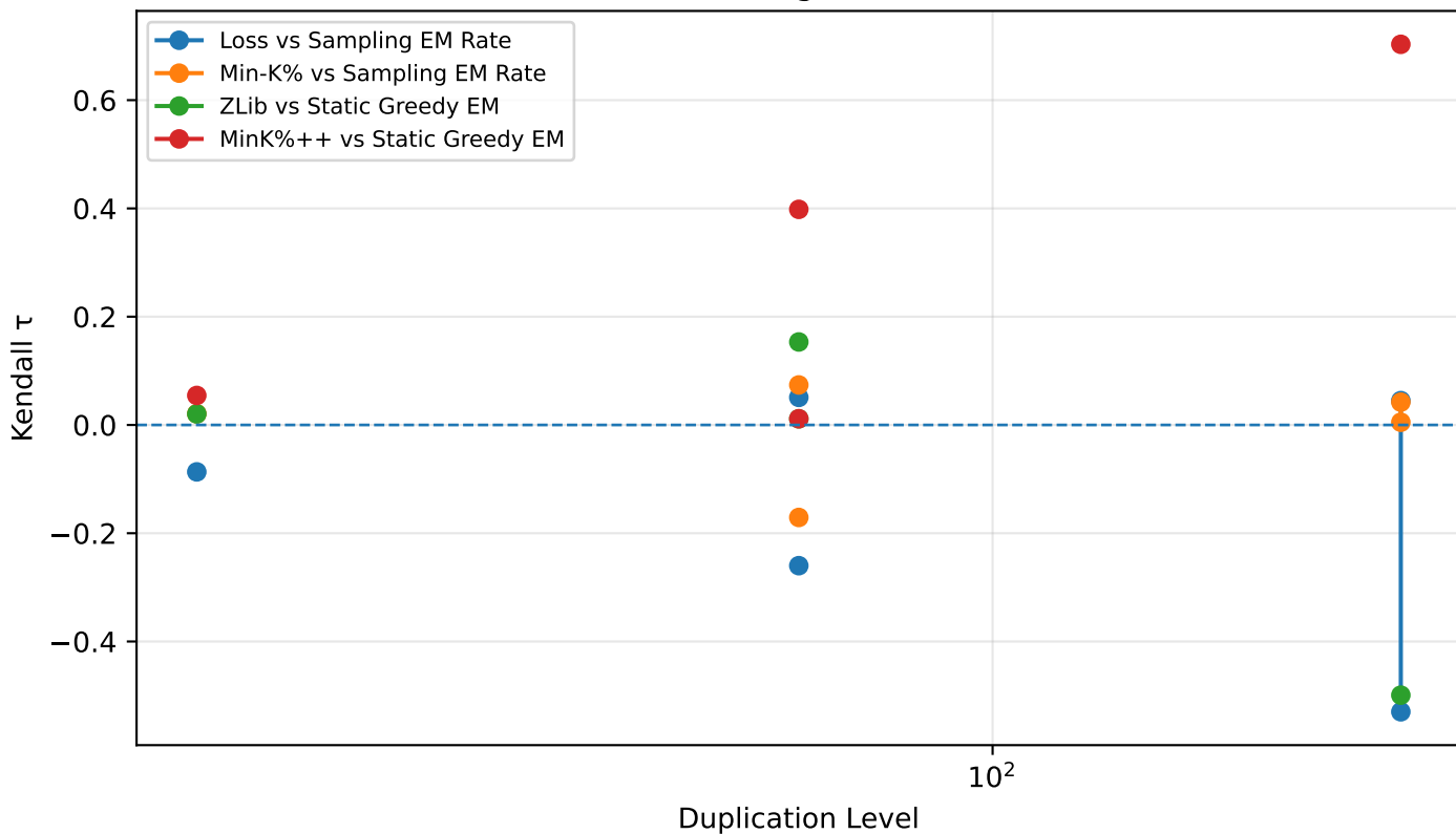
Correlation varies by duplication level target
