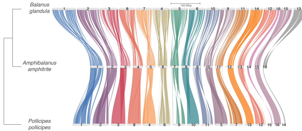
Figure 1: Conserved synteny across barnacle genomes.
