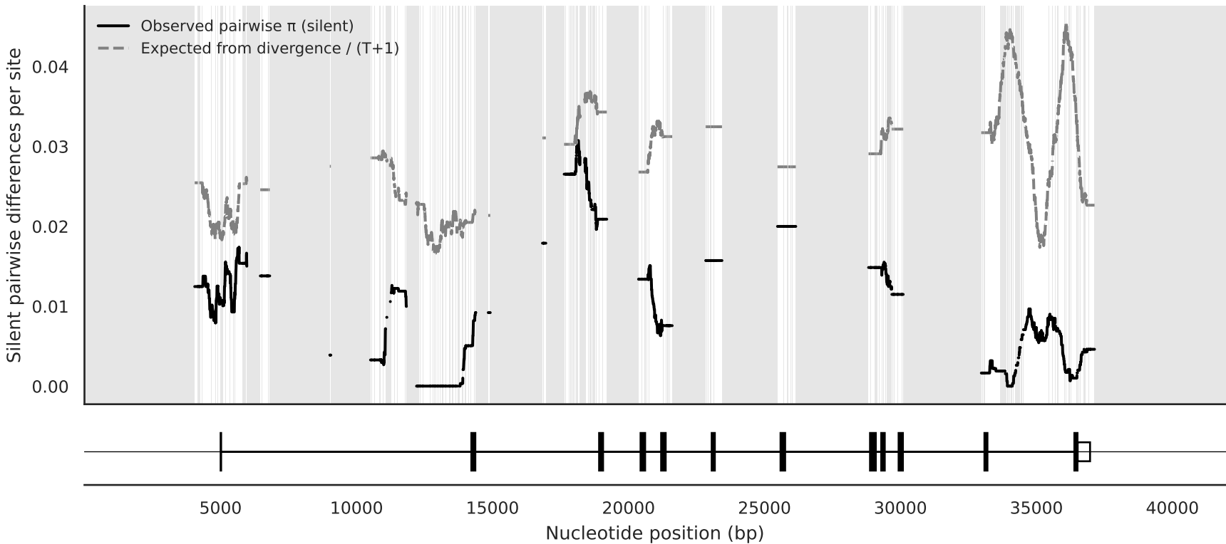
Me_1 — T+1=9.15, w=500 silent sites
