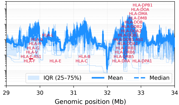
Chr6 - HLA region
