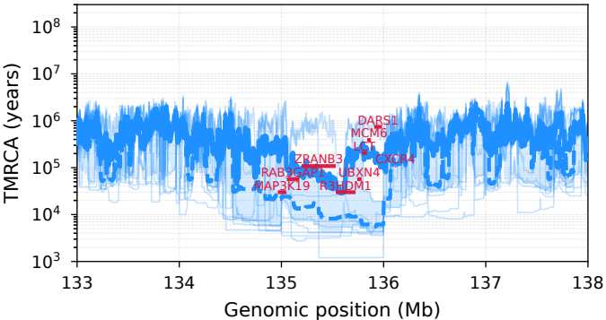
Chr2 - LCT locus
