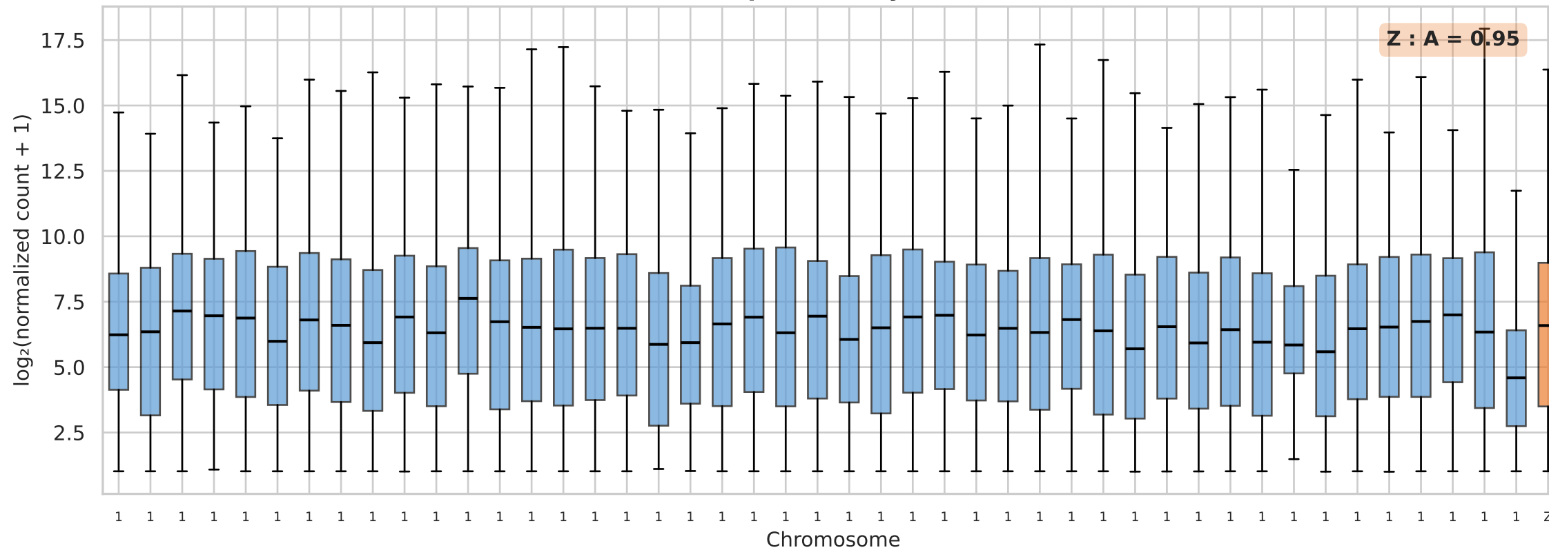
Male (ZZ) Expression by Chromosome
