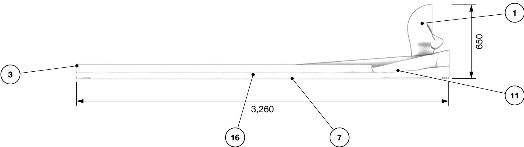
Side elevation, from the left
