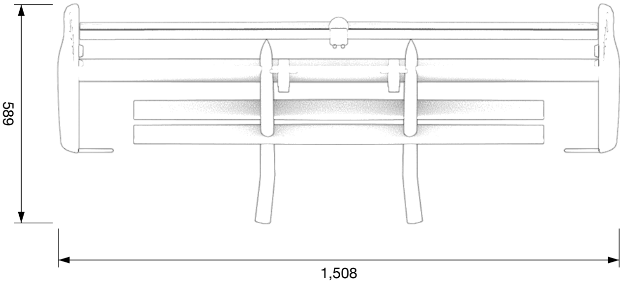
End view, from the nose
