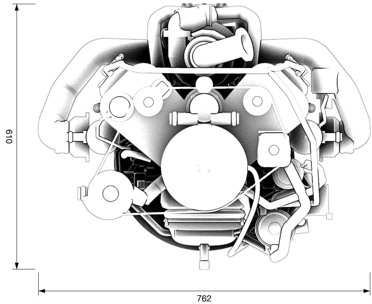
End view, from the nose
