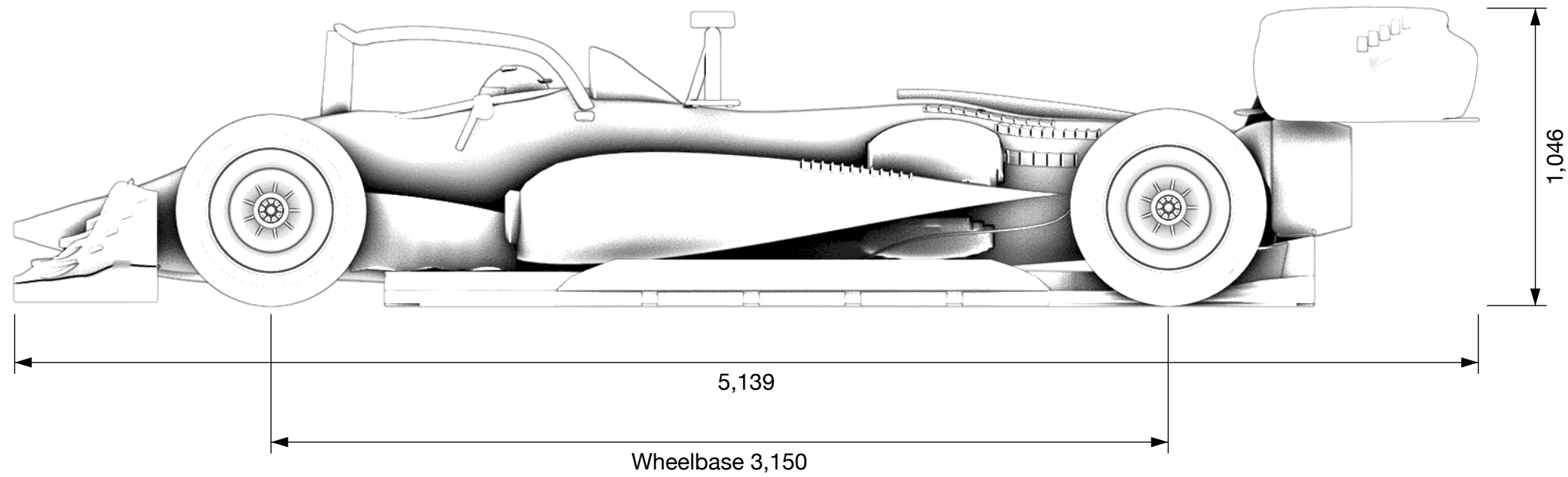
Side elevation, from the left
