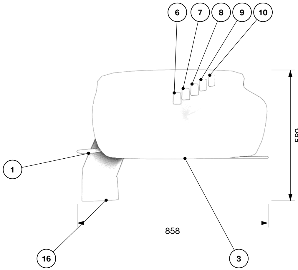
Side elevation, from the left
