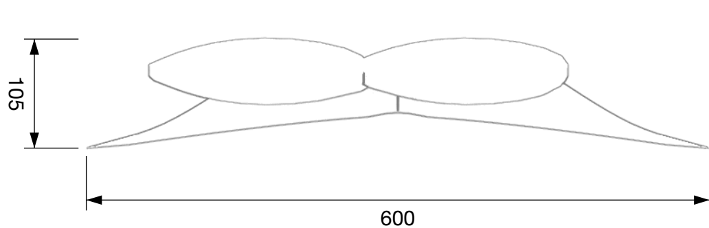
End view, from the nose
