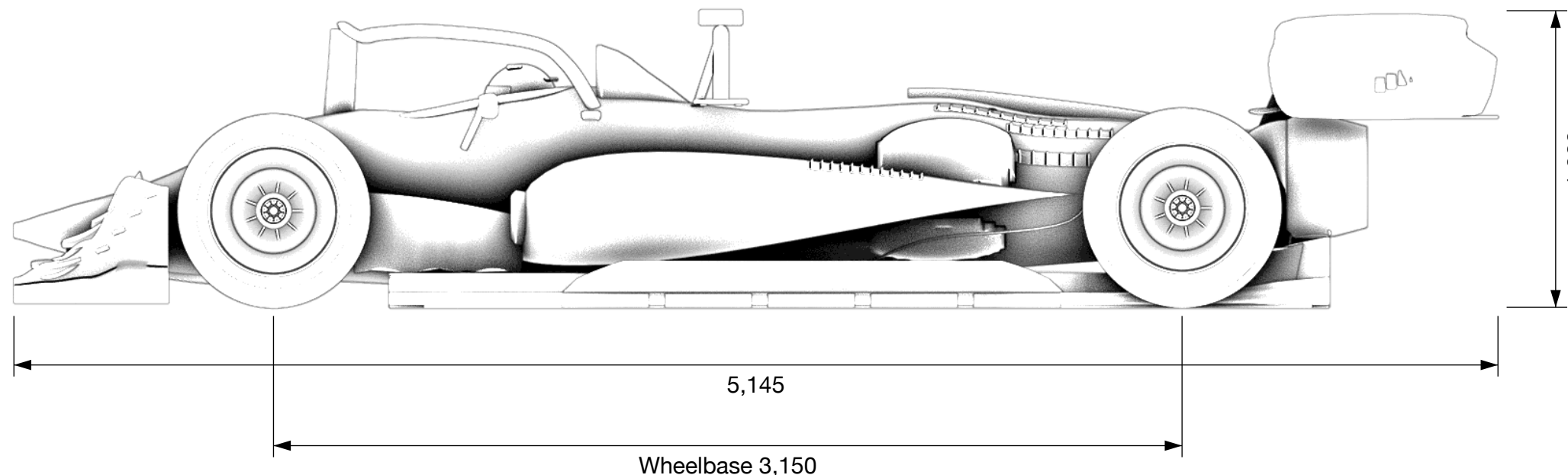
Side elevation, from the left
