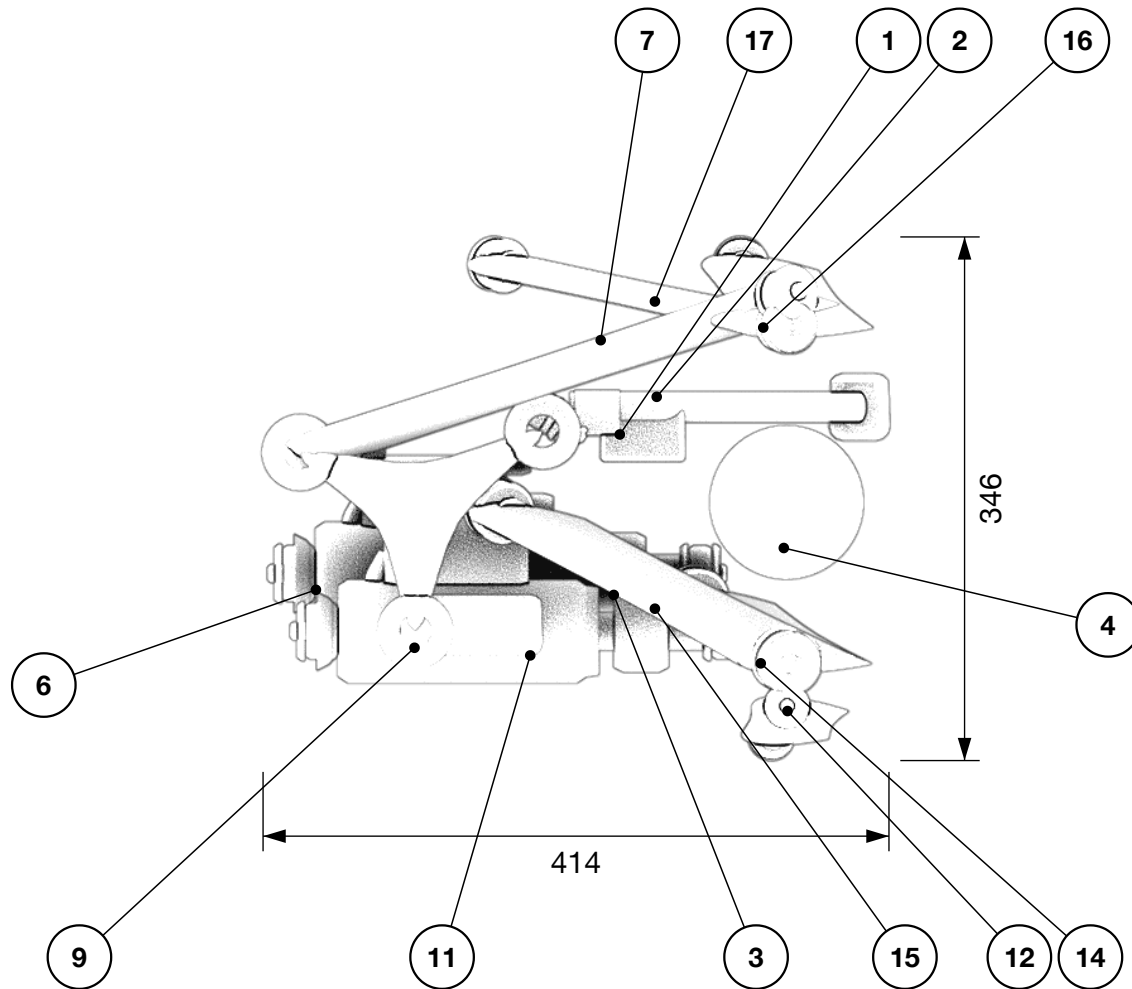
Side elevation, from the left
