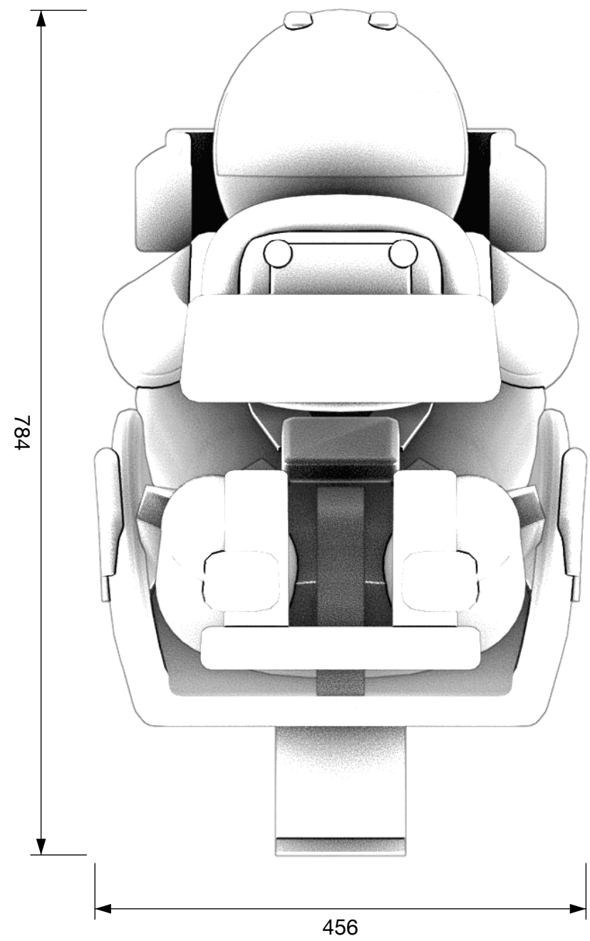
End view, from the nose
