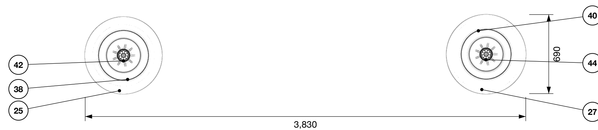
Side elevation, from the left
