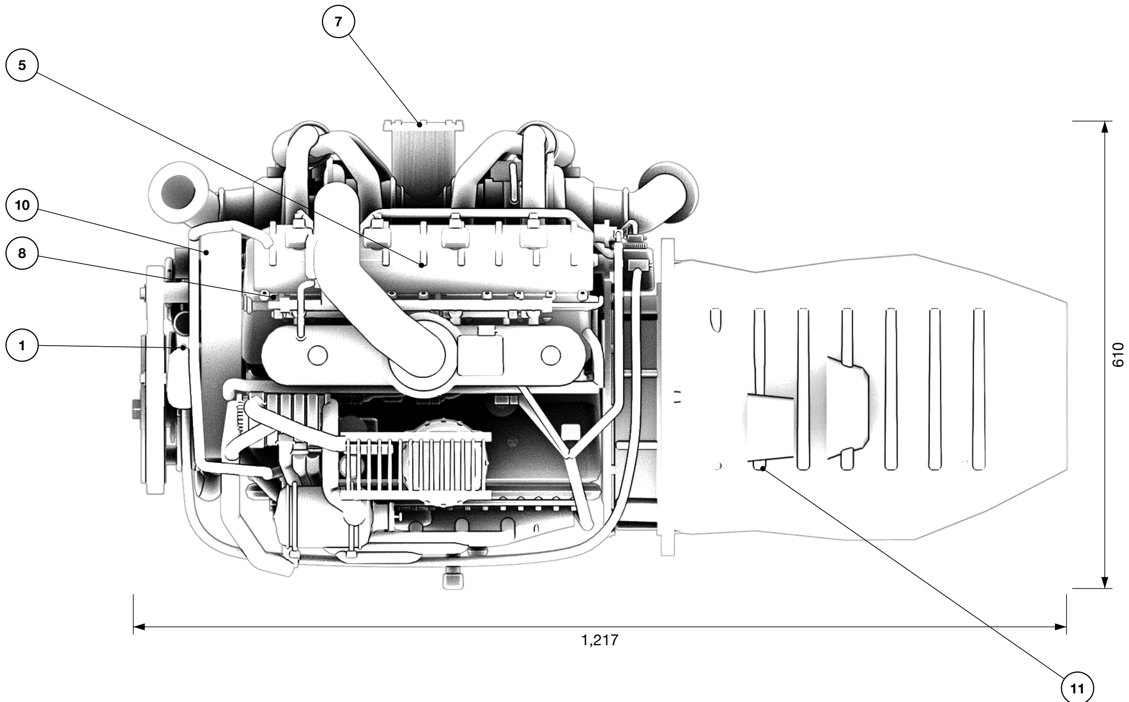
Side elevation, from the left
