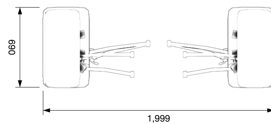
End view, from the nose
