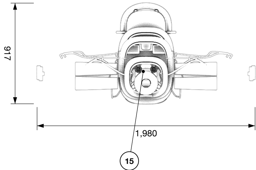
End view, from the nose
