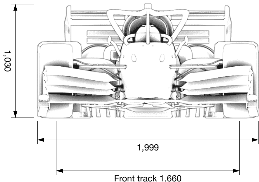
End view, from the nose
