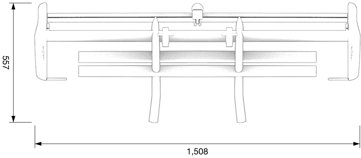
End view, from the nose
