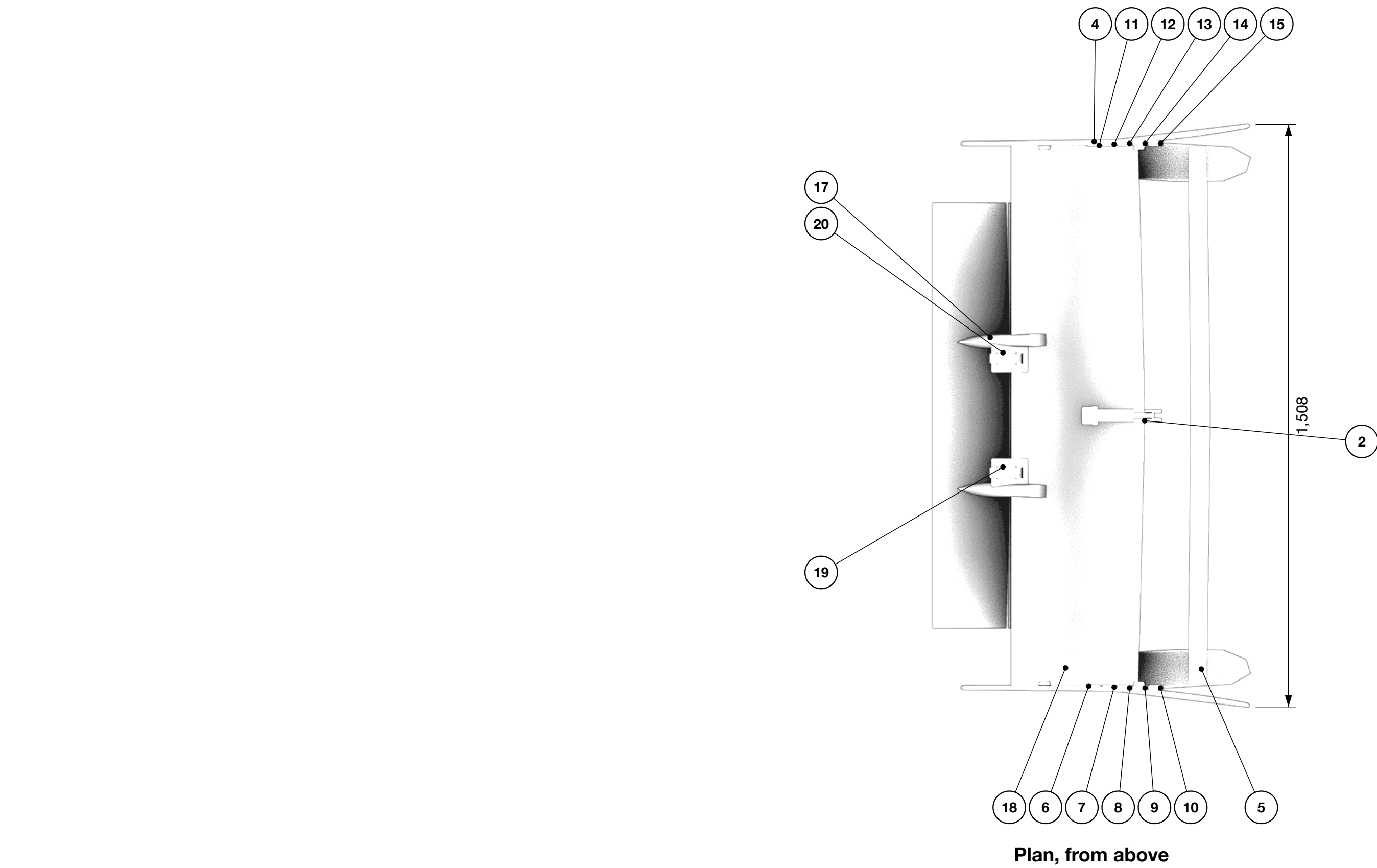
Plan, from above
