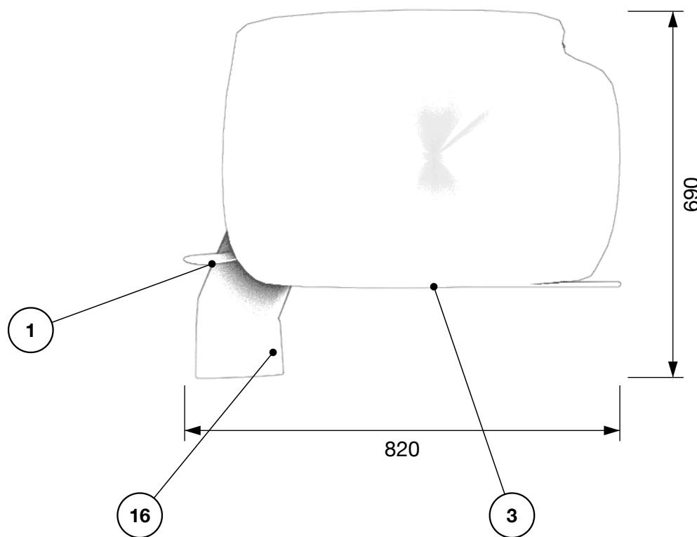
Side elevation, from the left
