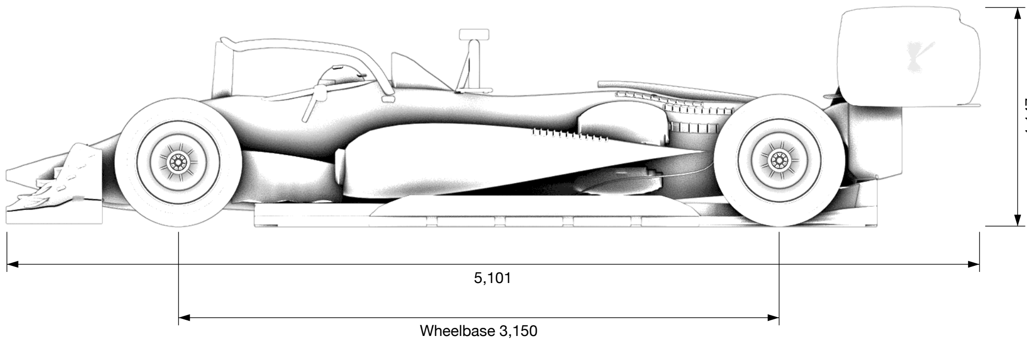
Side elevation, from the left
