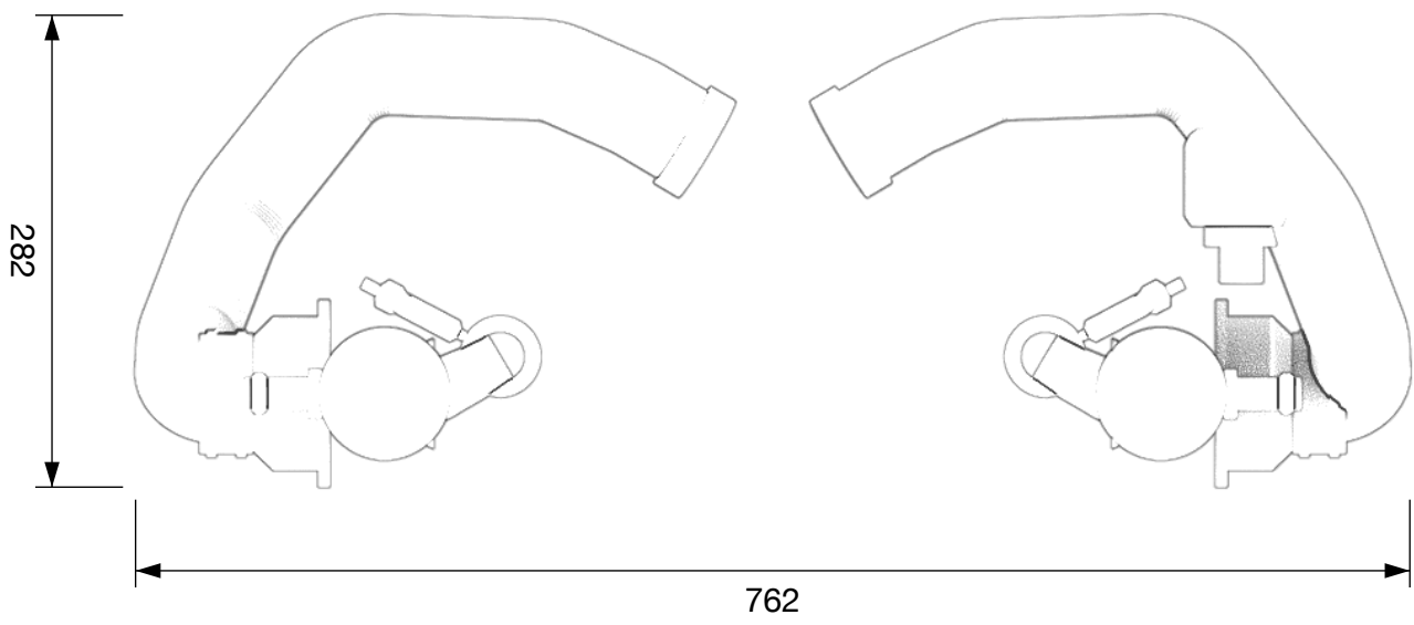
End view, from the timing end
