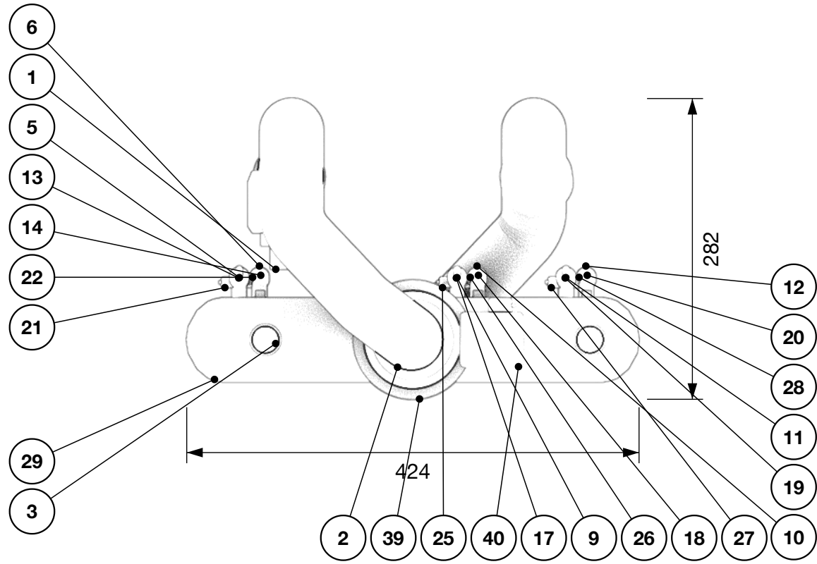
Side elevation, from the left
