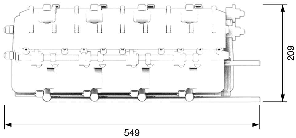
Side elevation, from the left
