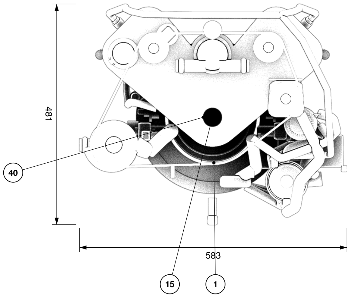
End view, from the timing end
