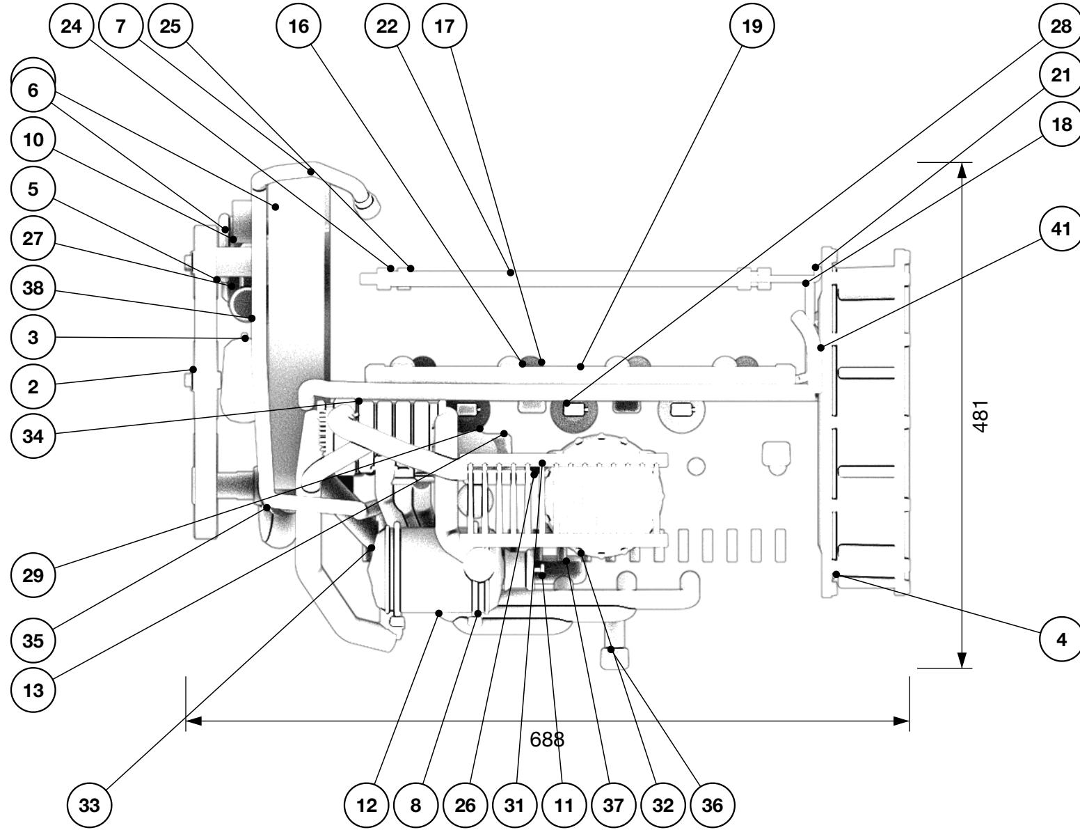
Side elevation, from the left
