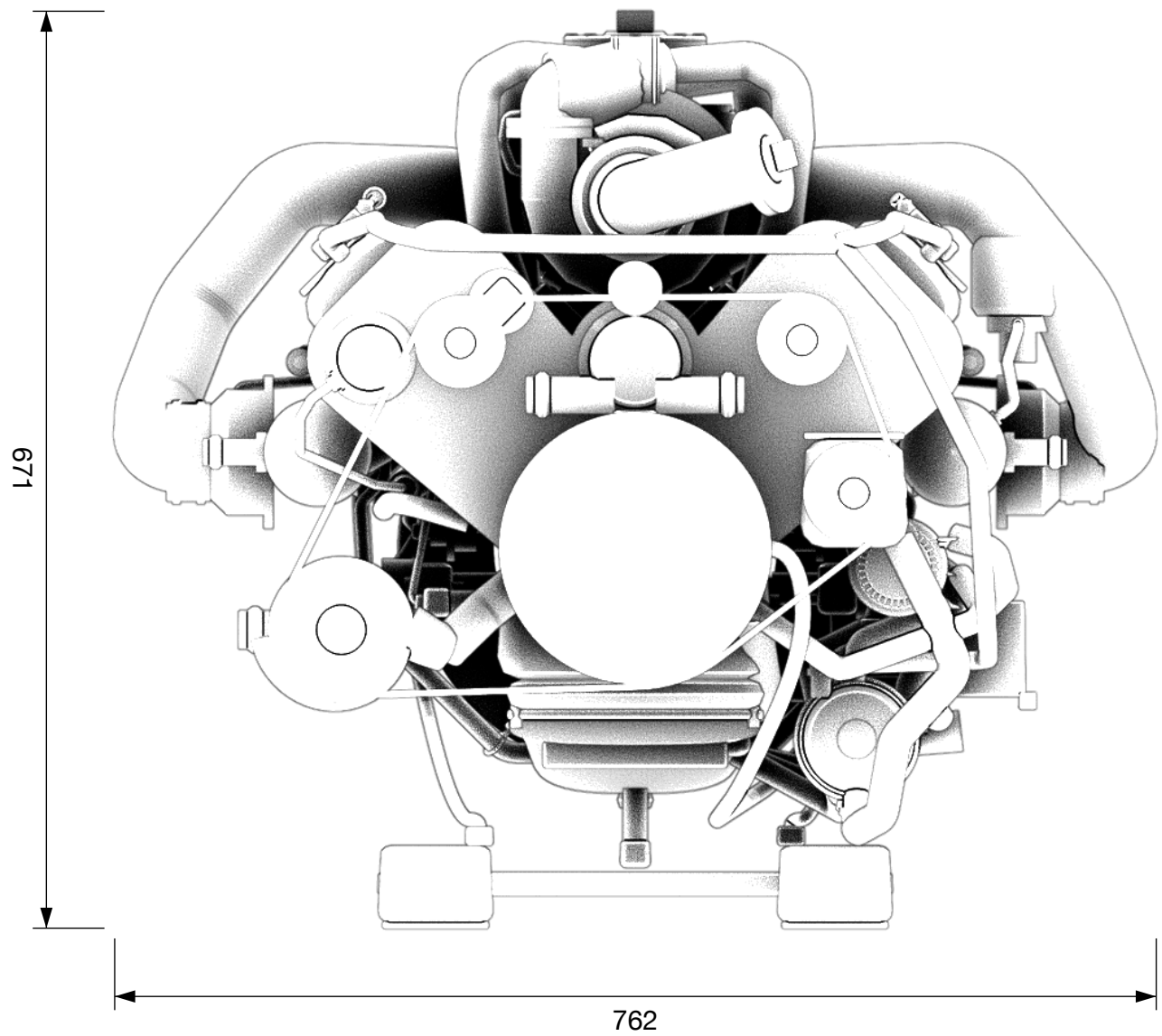
End view, from the timing end
