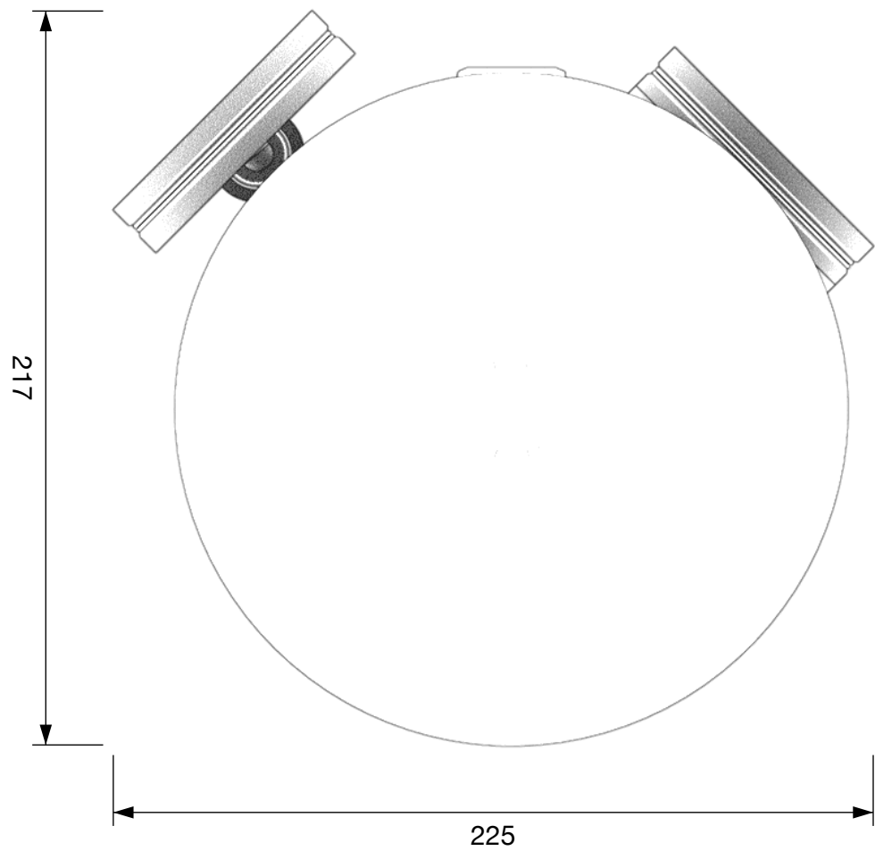
End view, from the timing end
