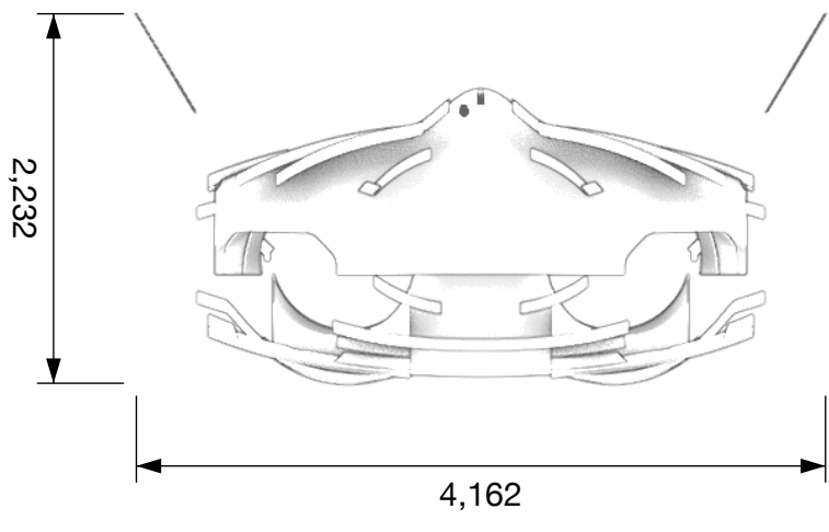
End view, from the nose
