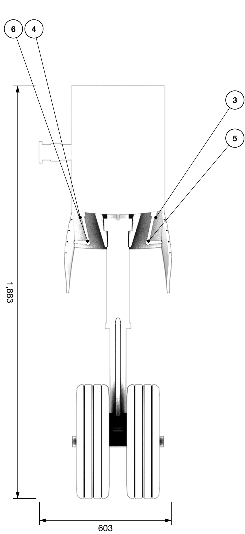
End view, from the nose
