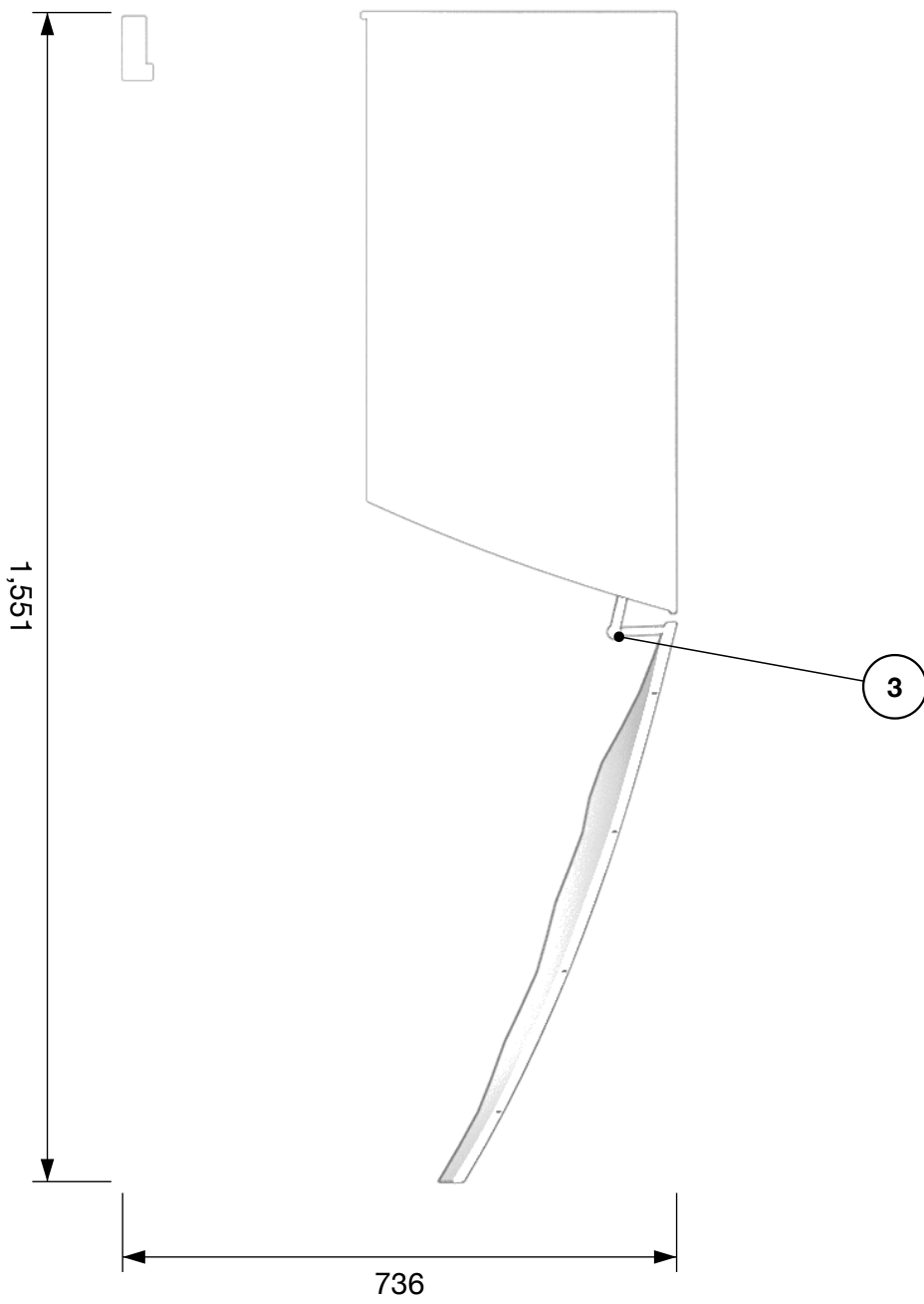
End view, from the nose
