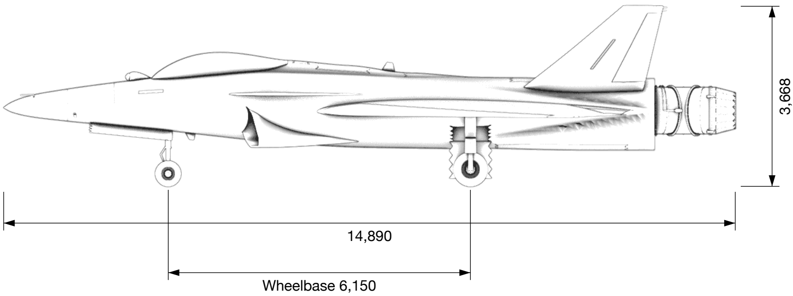
Side elevation, from the left
