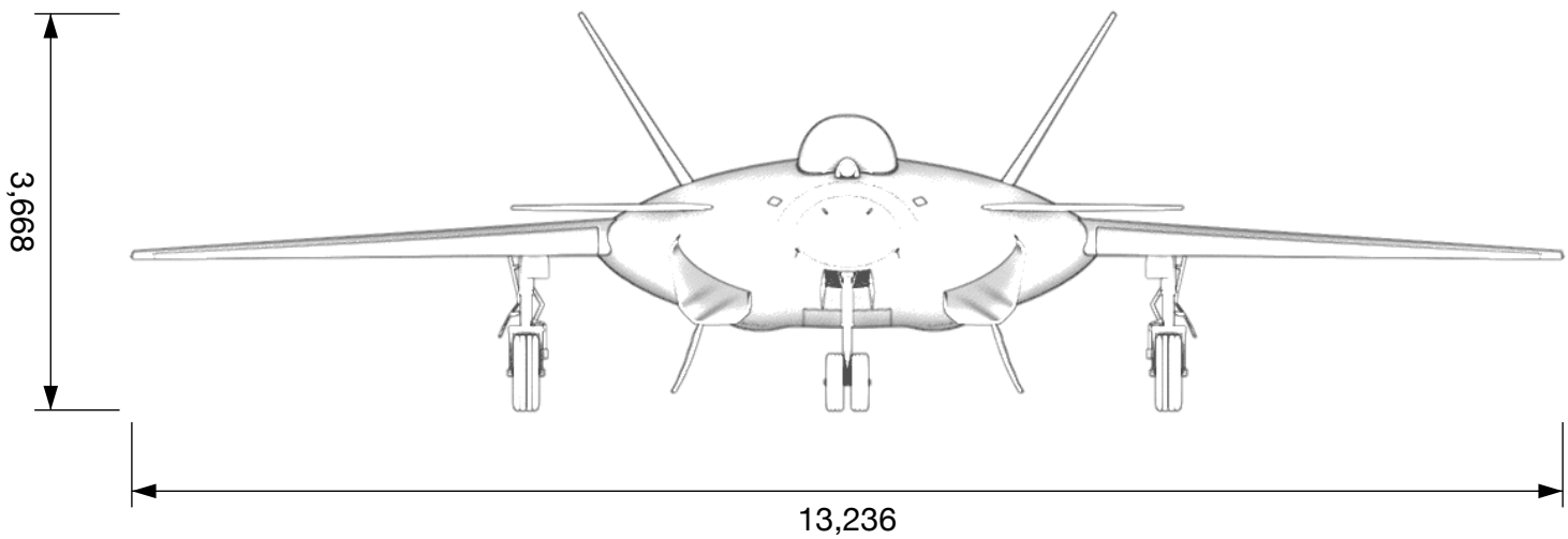
End view, from the nose
