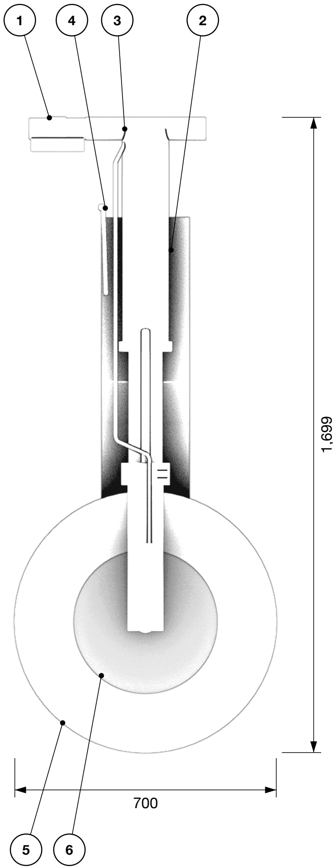
Side elevation, from the left
