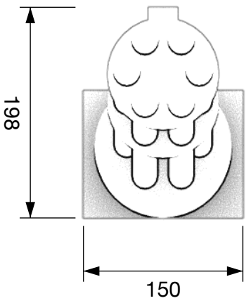
End view, from the nose
