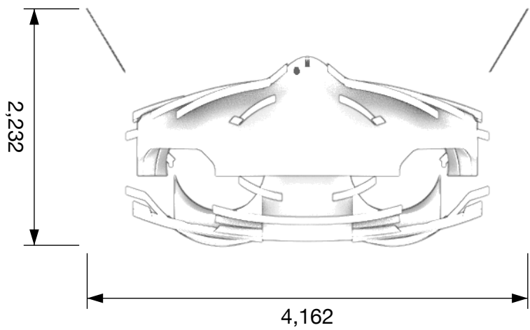
End view, from the nose
