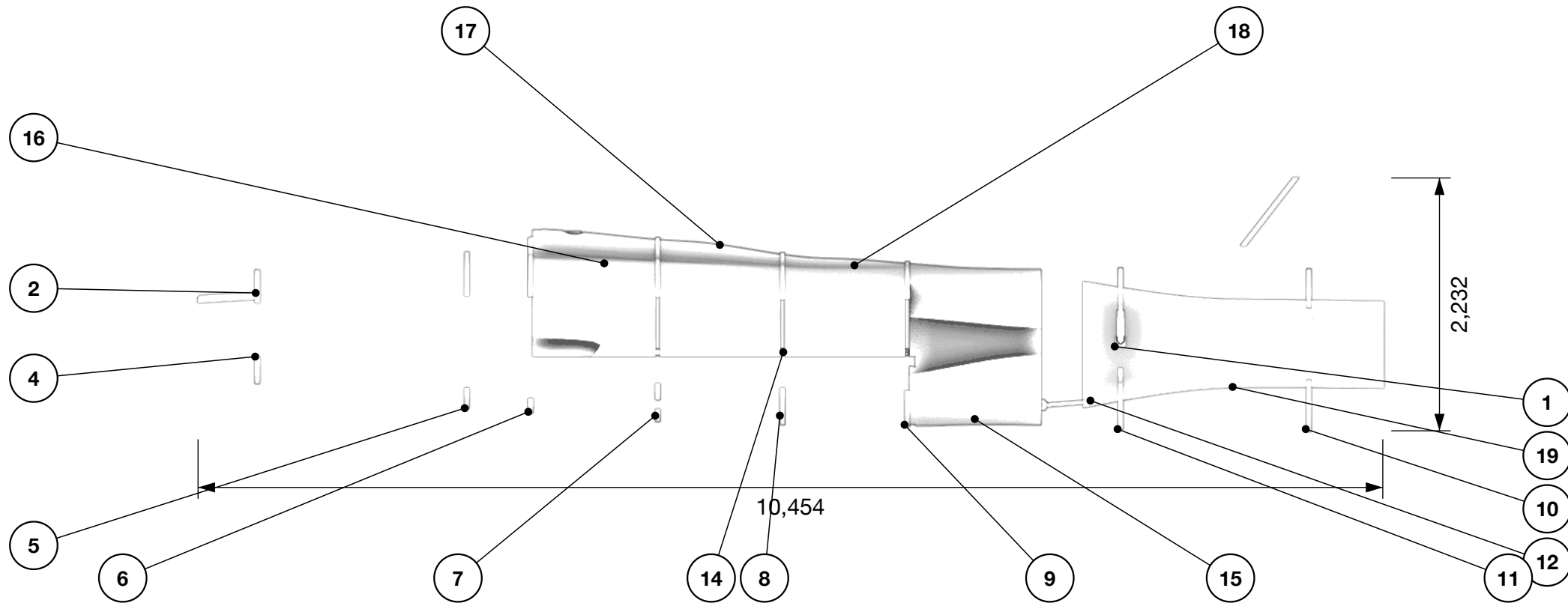
Side elevation, from the left
