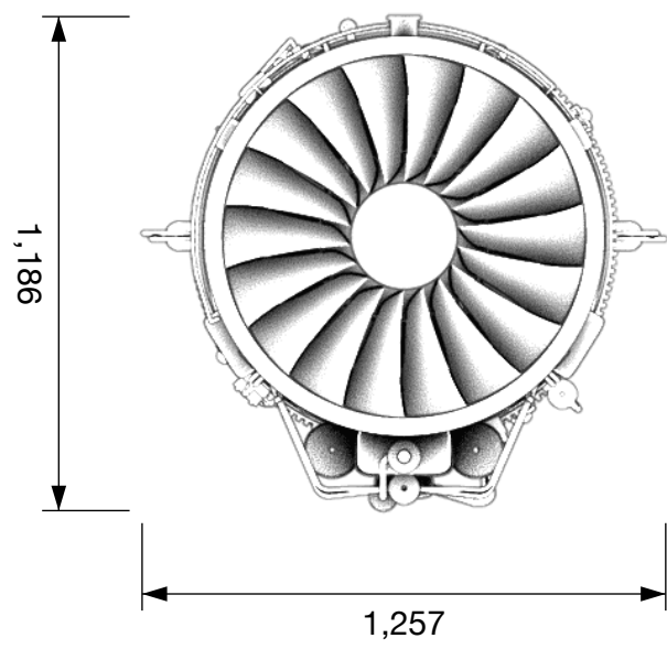
End view, from the nose
