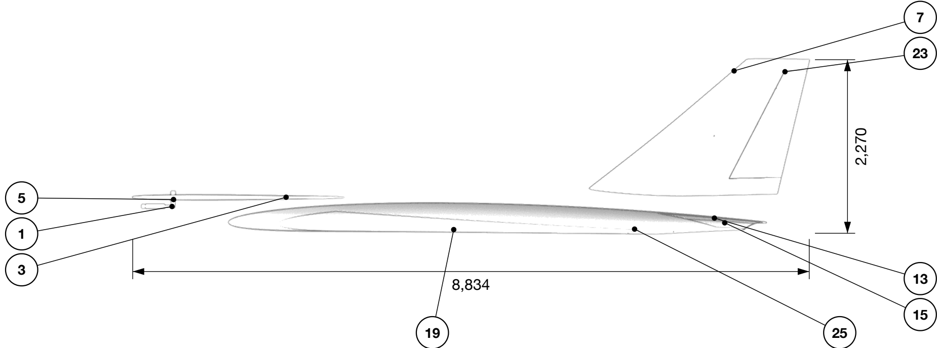
Side elevation, from the left
