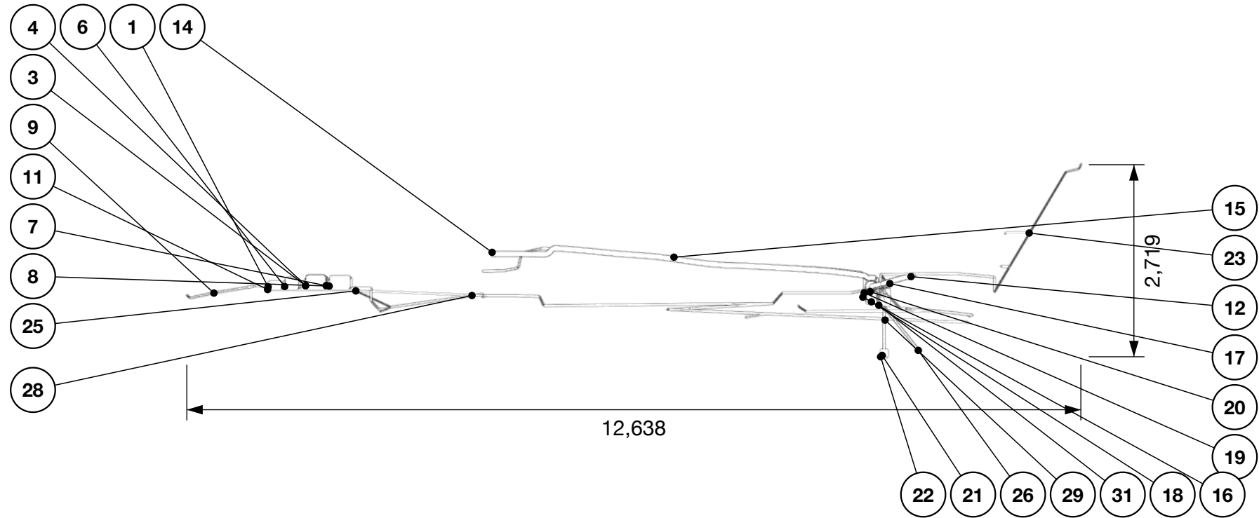
Side elevation, from the left
