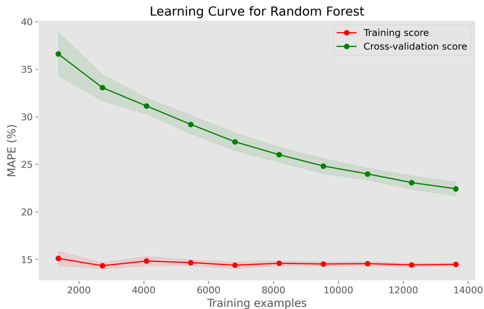
FIGURE 1.11: Learning curve for the random forest model. The narrowing gap between training and cross-validation MAPE suggests good generalization and that additional data may still yield incremental improvements.
