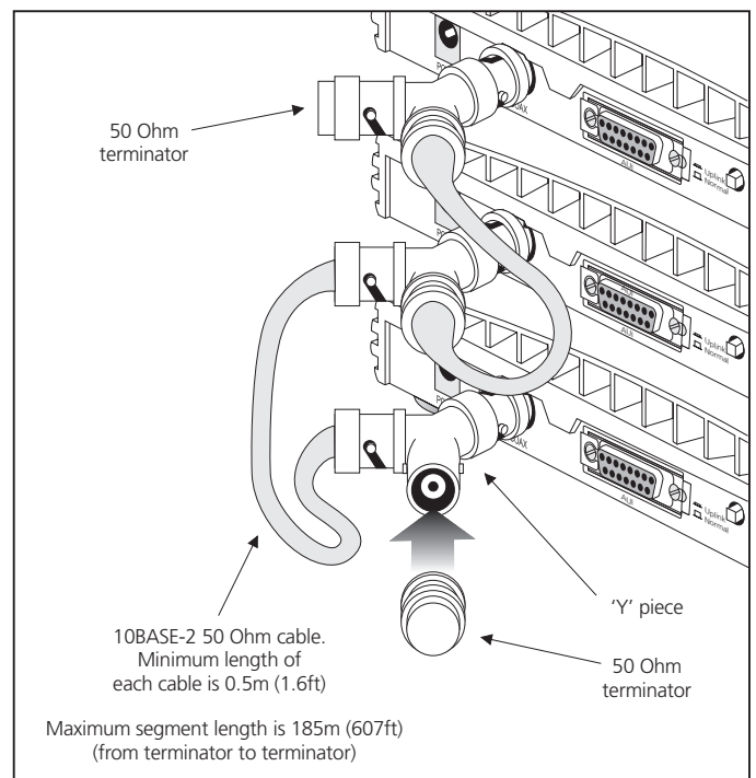
Figure 4 Correct Hub Connections Using 10BASE-2
