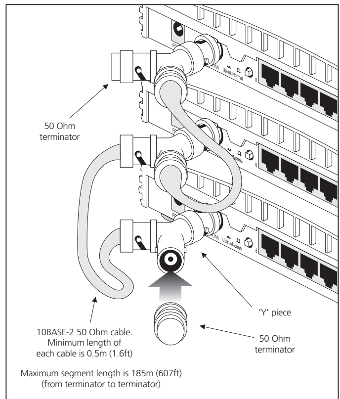
Figure 7 Correct Hub Connections Using 10BASE-2
