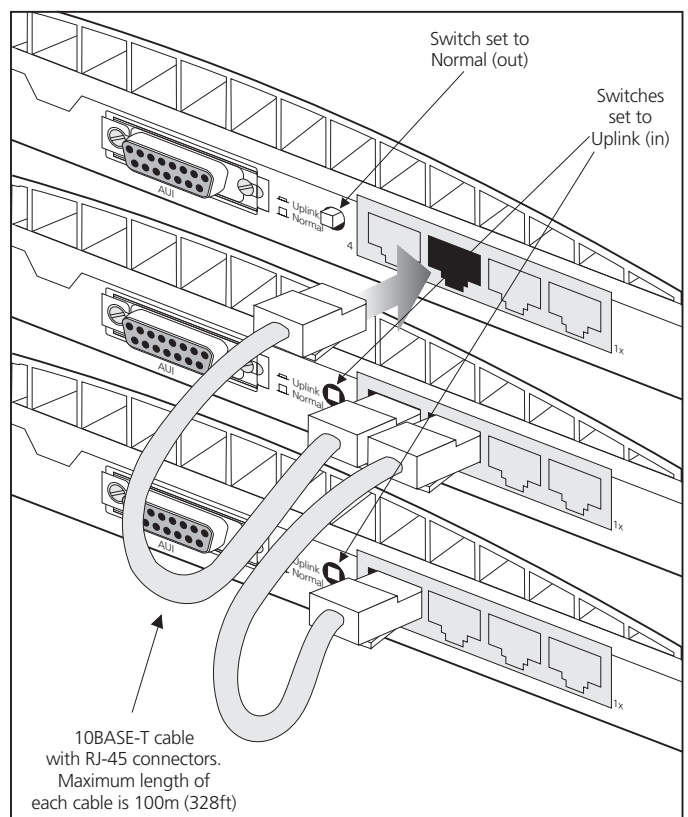
Figure 5 Correct Hub Connections Using 10BASE-T
