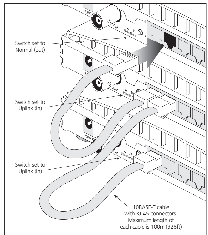
Figure 8 Correct Hub Connections Using 10BASE-T
