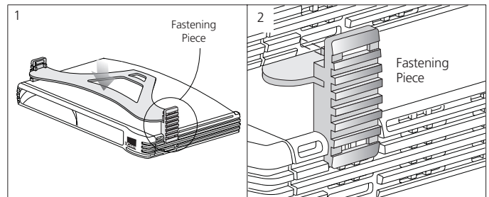
Figure 3 Stacking Your Units Together
