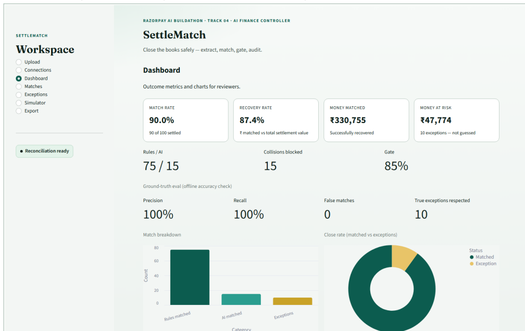
Fig 8 - Dashboard after the live run (90 matched, 10 exceptions).
