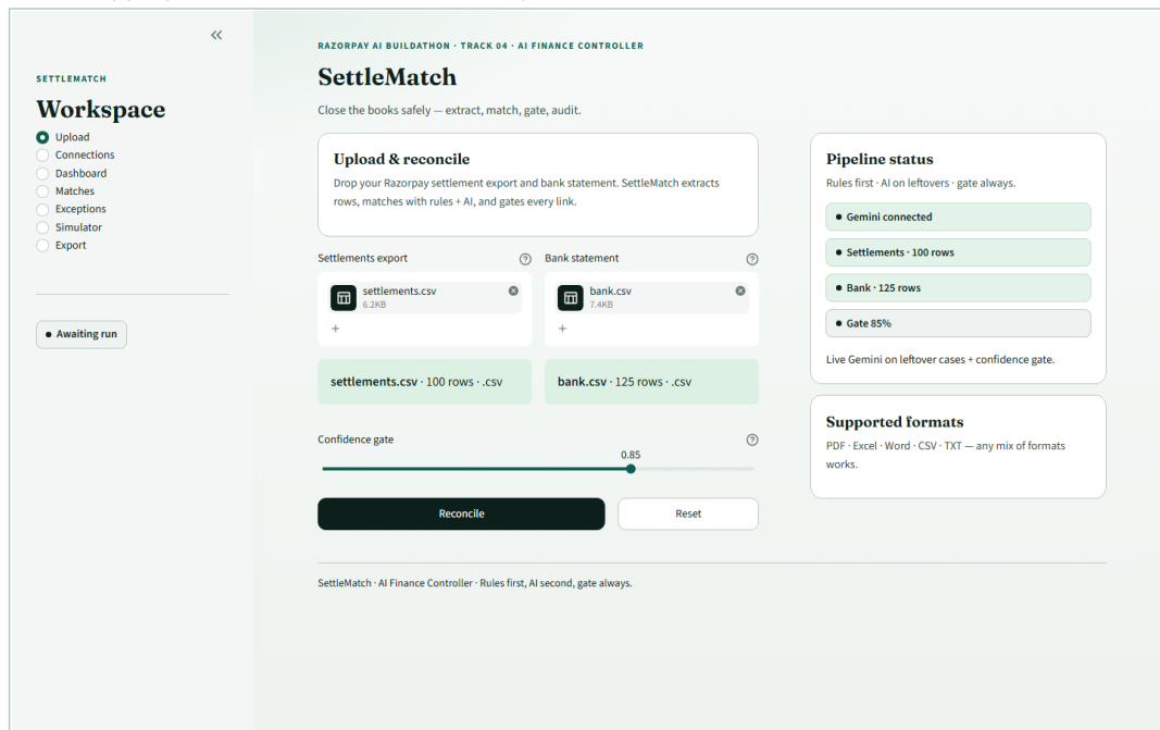
Fig 6 - Upload with both sample files extracted. Reconcile is enabled.
