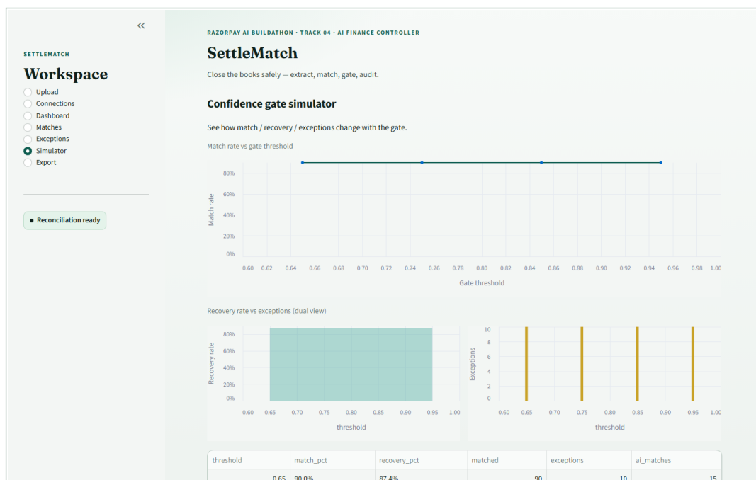
Fig 11 - Gate simulator after reconciliation (not the empty-state page).
