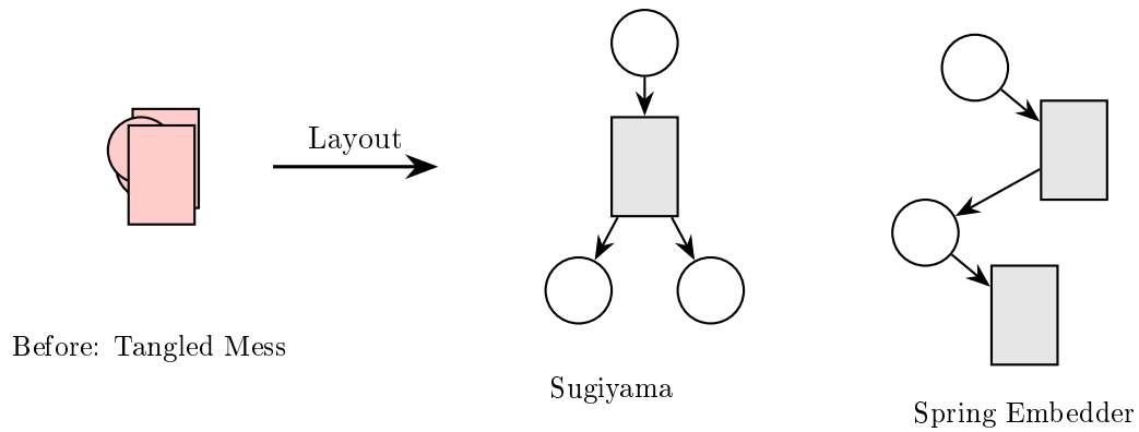
Figure 6.1: Layout transforms tangled nodes into readable graphs
