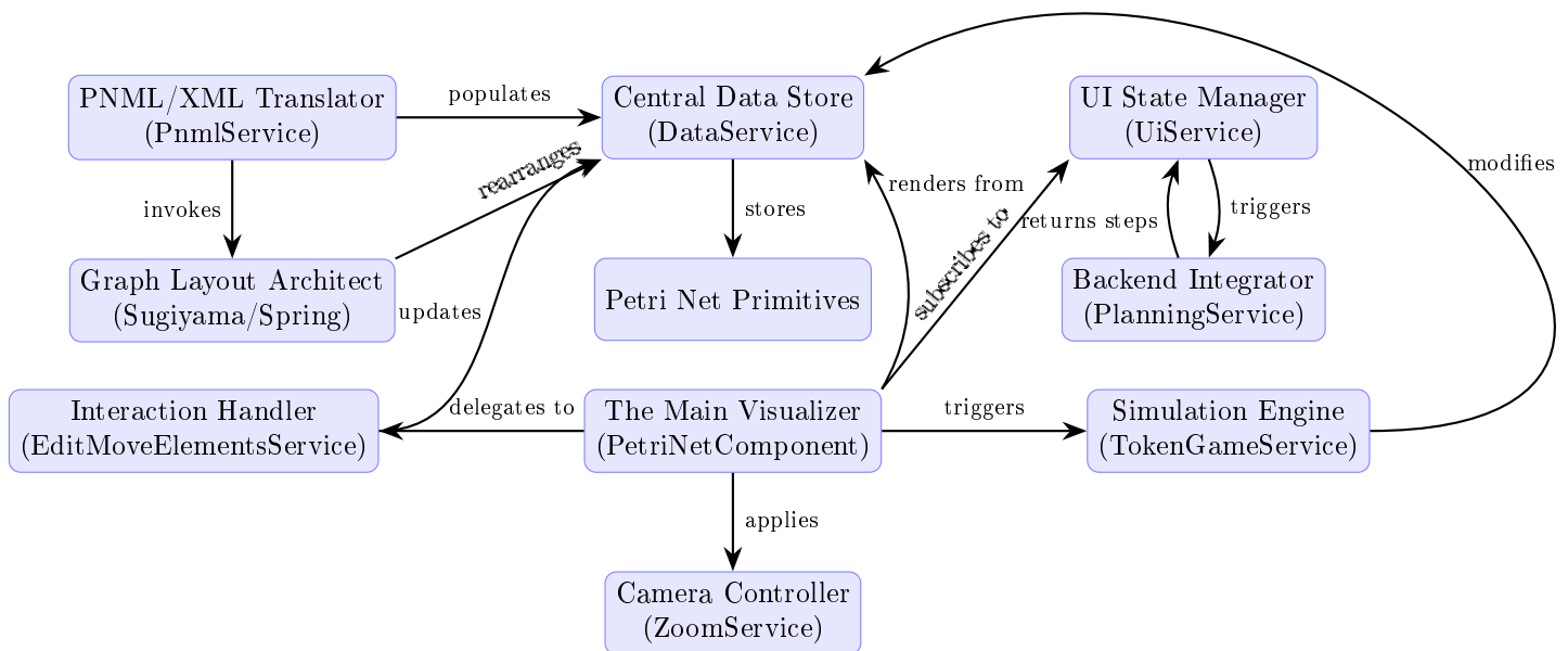
Figure 1.1: PNML_Frontend System Architecture
