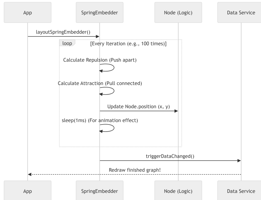
Figure 6.2: Sequence Diagram: Spring Embedder Physics Loop
