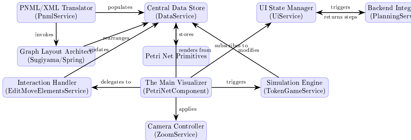
Figure 1.1: PNML_Frontend System Architecture
