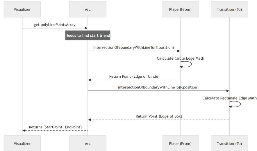
Figure 2.2: Sequence Diagram: Arc requests boundary intersection points
