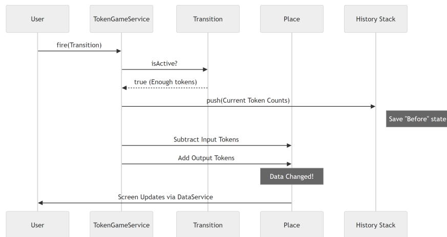
Figure 10.3: Sequence Diagram: Token Game Firing Logic
