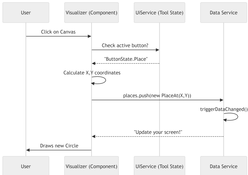
Figure 4.2: Sequence Diagram: Creating a Place via Click
