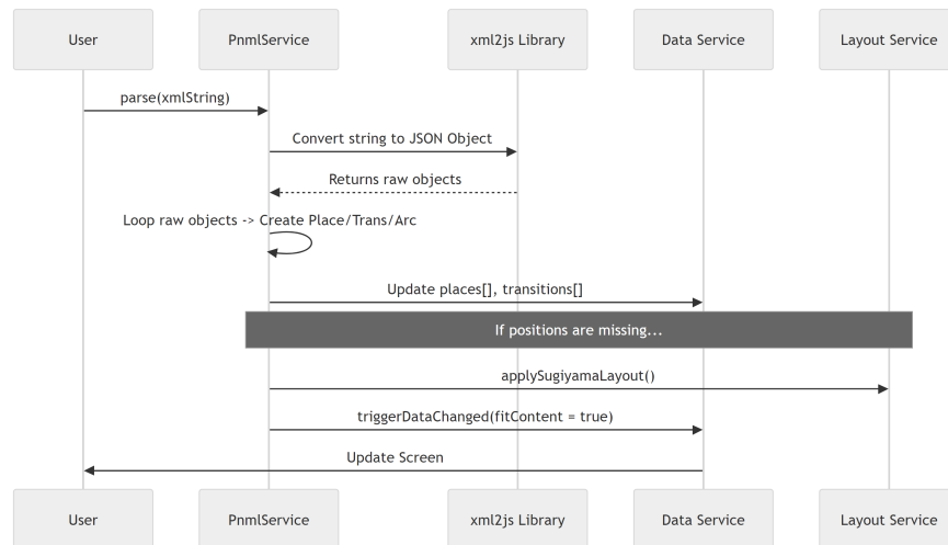
Figure 5.2: Sequence Diagram: PNML Import Process
