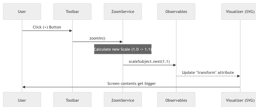
Figure 8.2: Sequence Diagram: Zoom In via Toolbar Button
