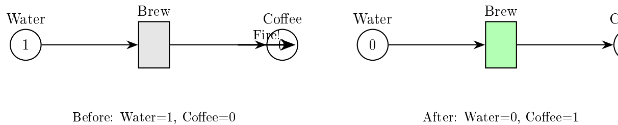
Figure 10.1: Firing a Transition: Tokens move from input to output places
