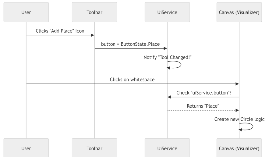
Figure 9.2: Sequence Diagram: Tool Selection and Place Creation
