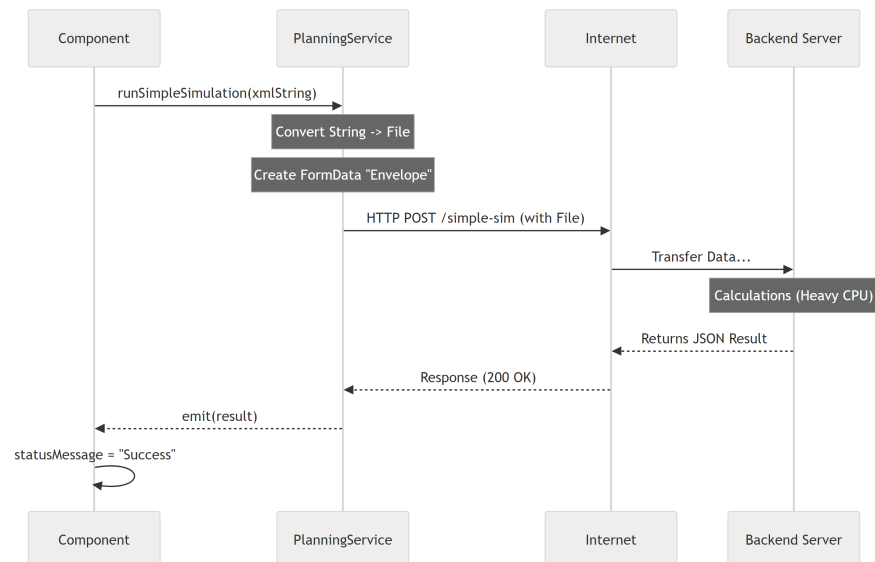
Figure 11.2: Sequence Diagram: Running a Backend Simulation
