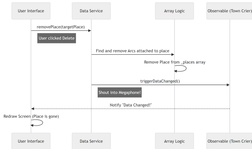
Figure 3.2: Sequence Diagram: Deleting a Place triggers cascading updates
