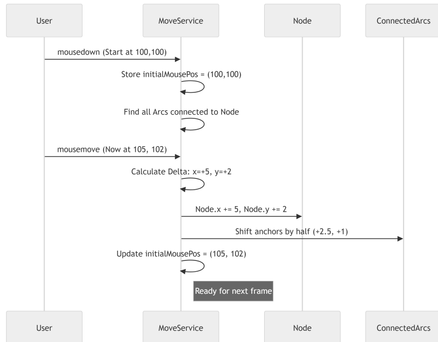
Figure 7.3: Sequence Diagram: Dragging a Node with Connected Arcs
