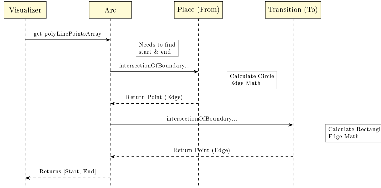
Figure 2.2: Sequence Diagram: Arc requests boundary intersection points
