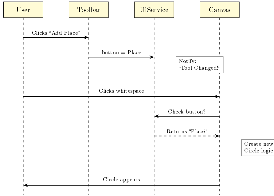
Figure 9.2: Sequence Diagram: Tool Selection and Place Creation
