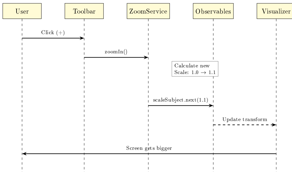
Figure 8.2: Sequence Diagram: Zoom In via Toolbar Button
