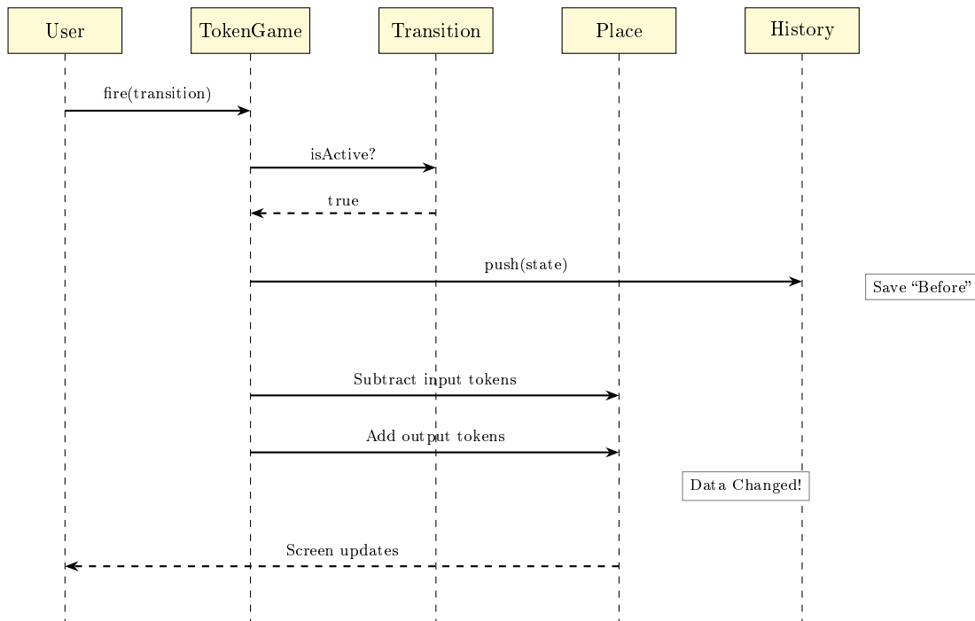
Figure 10.3: Sequence Diagram: Token Game Firing Logic
