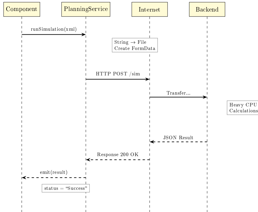
Figure 11.2: Sequence Diagram: Running a Backend Simulation
