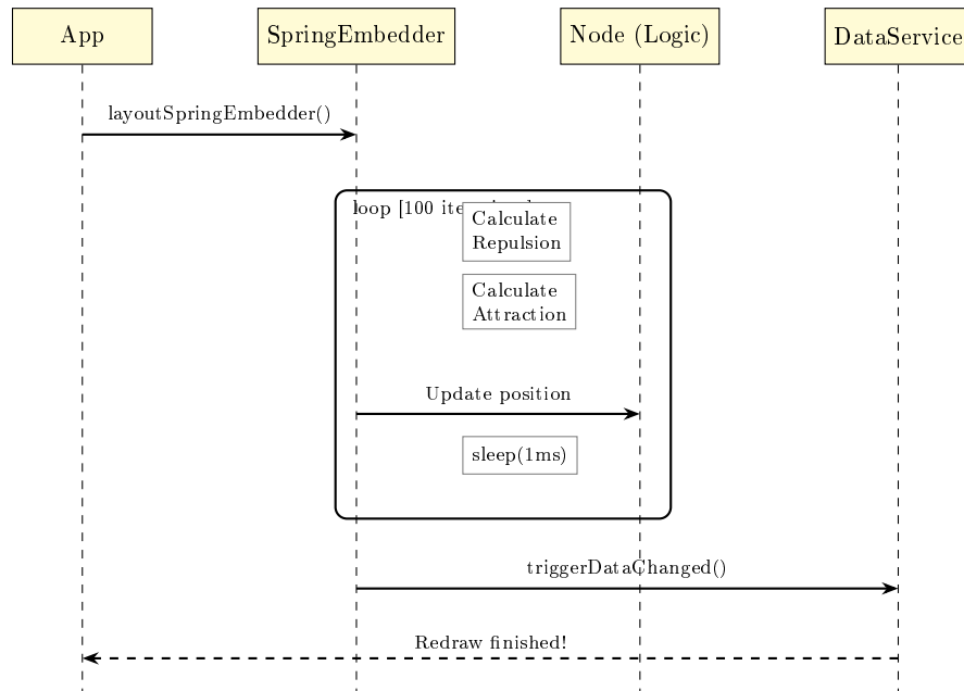
Figure 6.2: Sequence Diagram: Spring Embedder Physics Loop
