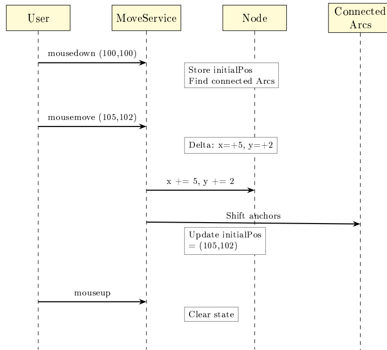
Figure 7.3: Sequence Diagram: Dragging a Node with Connected Arcs
