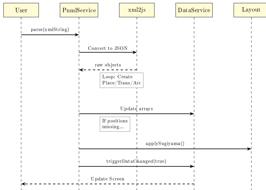
Figure 5.2: Sequence Diagram: PNML Import Process
