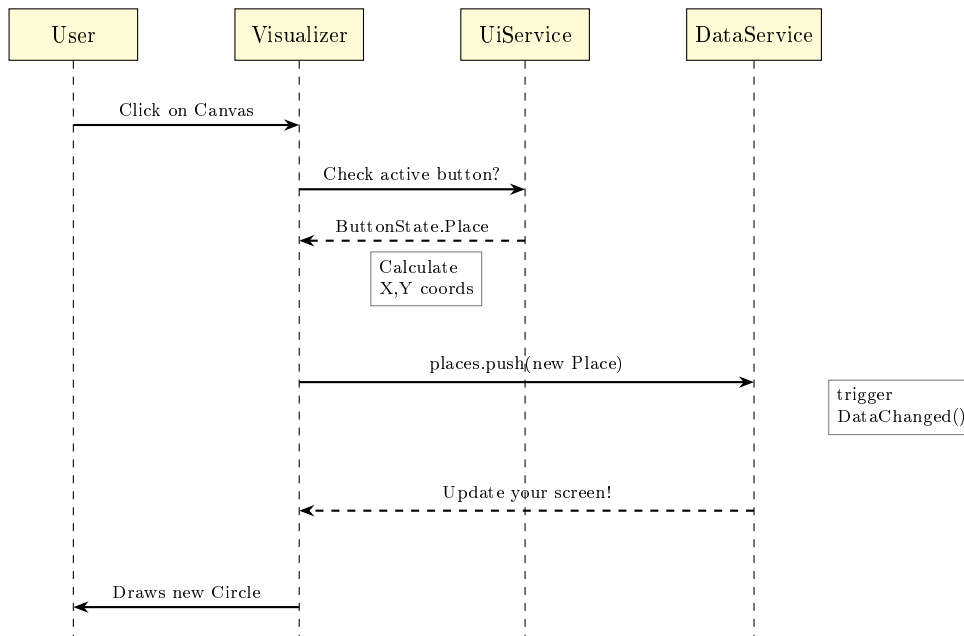
Figure 4.2: Sequence Diagram: Creating a Place via Click
