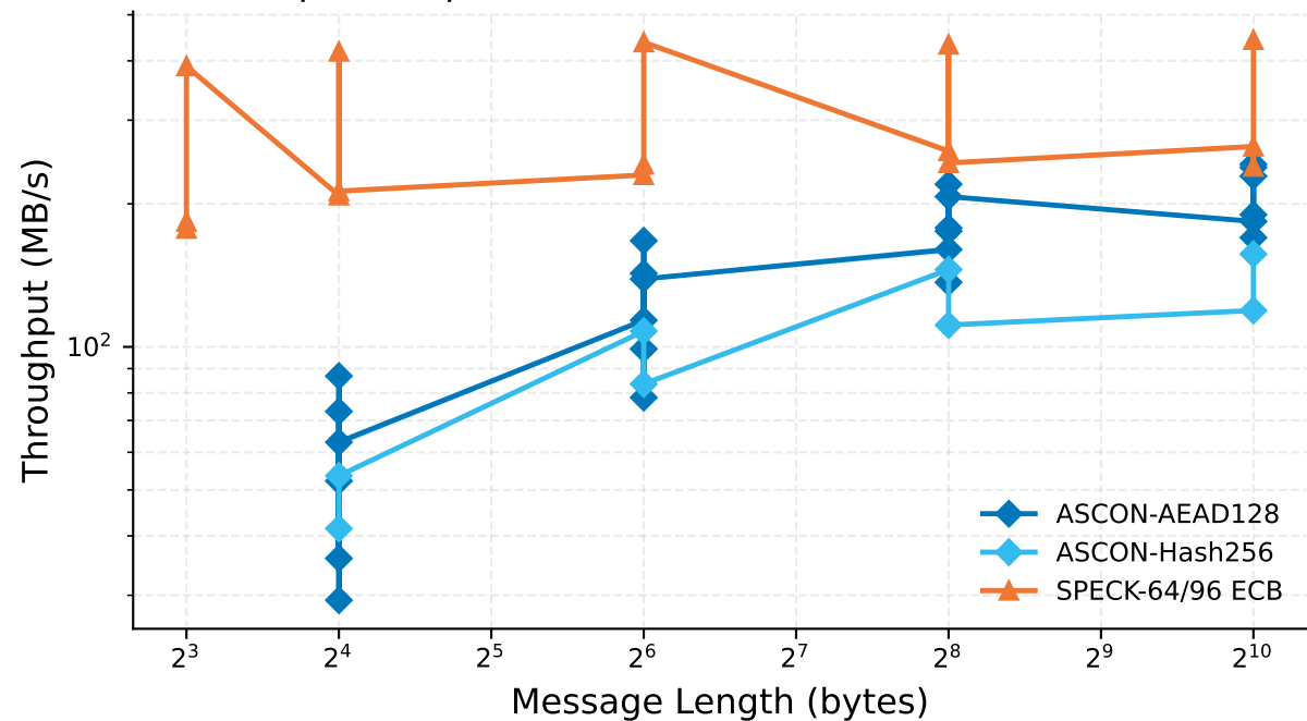
Fast Cipher Representatives: ASCON vs. SPECK-64/96 ECB
