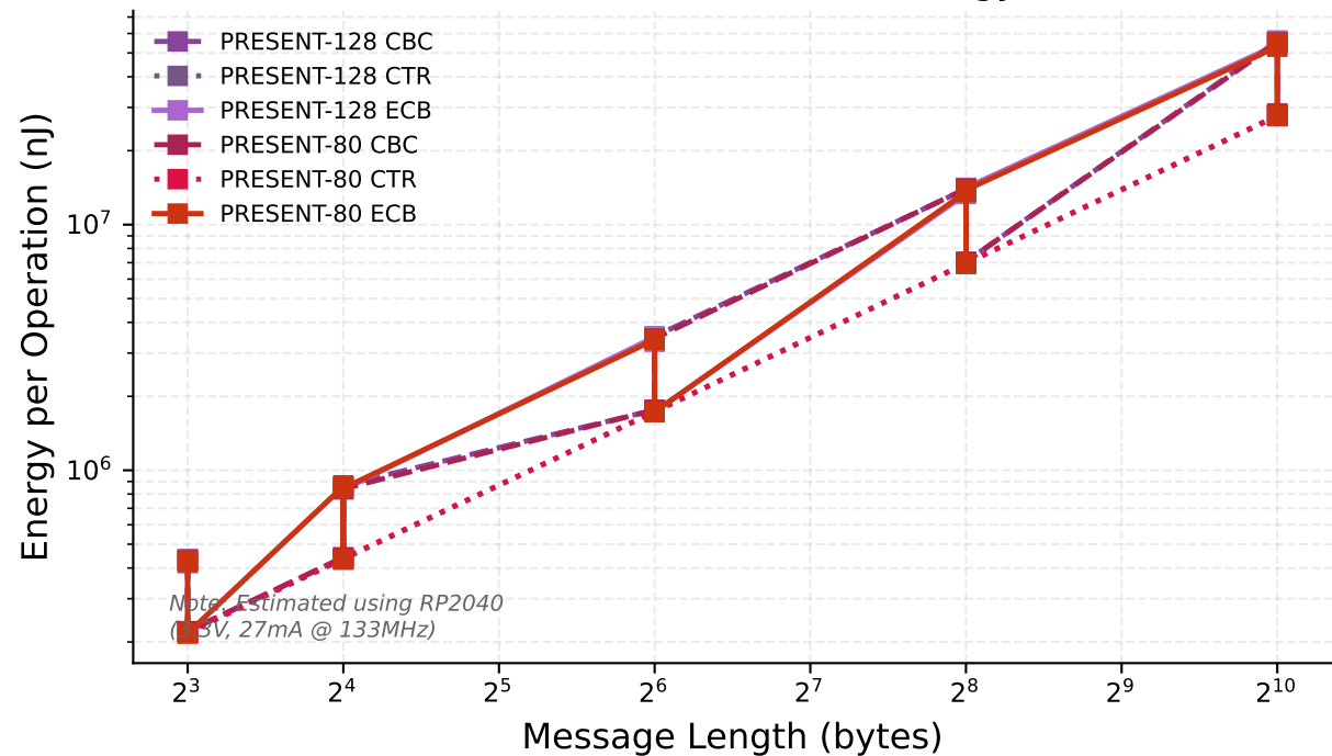
PRESENT — Estimated Energy
