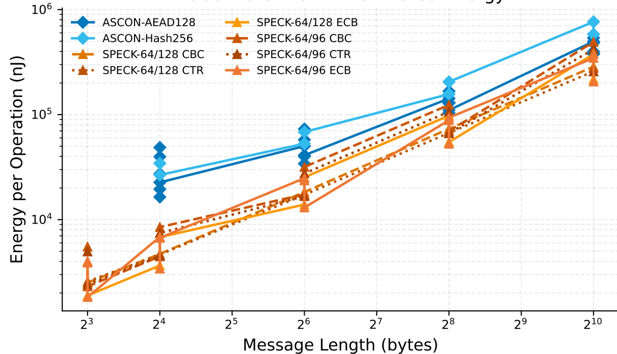
ASCON & SPECK — Estimated Energy
