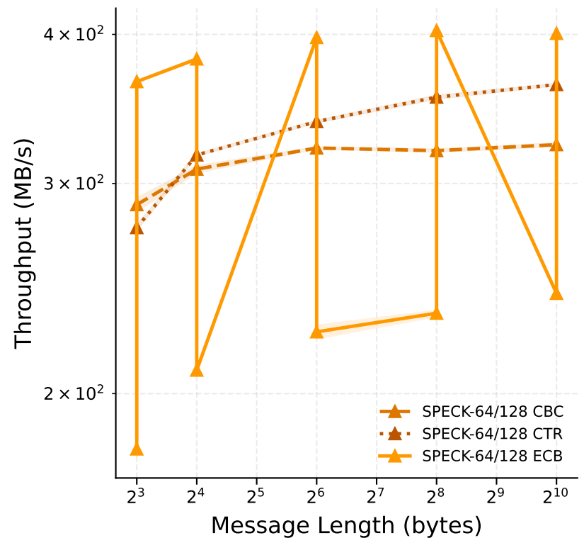
SPECK-64/128 Mode Overhead
