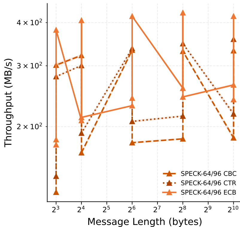
SPECK-64/96 Mode Overhead
