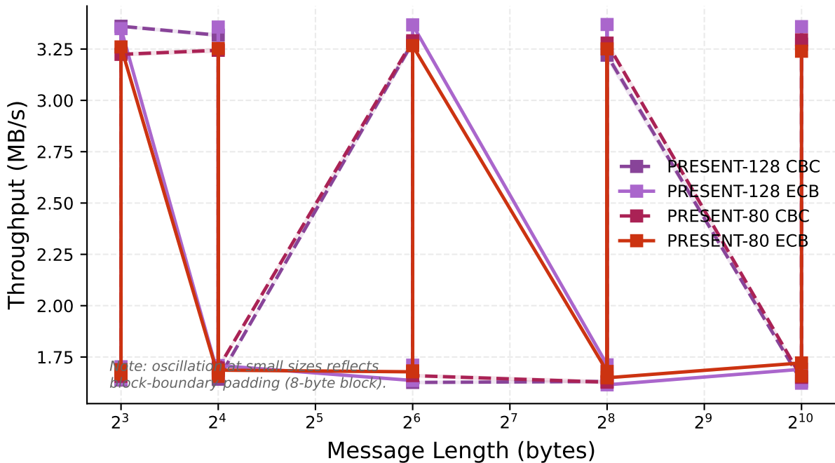
PRESENT: Key Size & Mode Comparison
