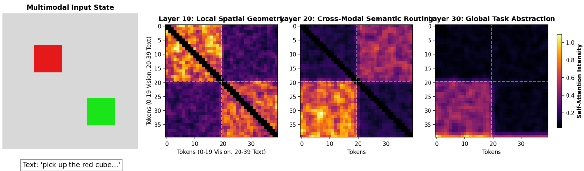
Figure 3: Evolution of Self-Attention across SmoIVLM layers. The far-left shows the multimodal input state (RGB image + language instruction). Layer 10 exhibits local spatial geometry. Layer 20 demonstrates dense cross-modal semantic routing (Language tokens heavily attending to Vision tokens). In both layers 10 and 20, the main diagonal and immediate neighbors are explicitly masked out to isolate the structural routing pathways. Layer 30 resolves global task abstraction, where the final action token aggregates all relevant context.
