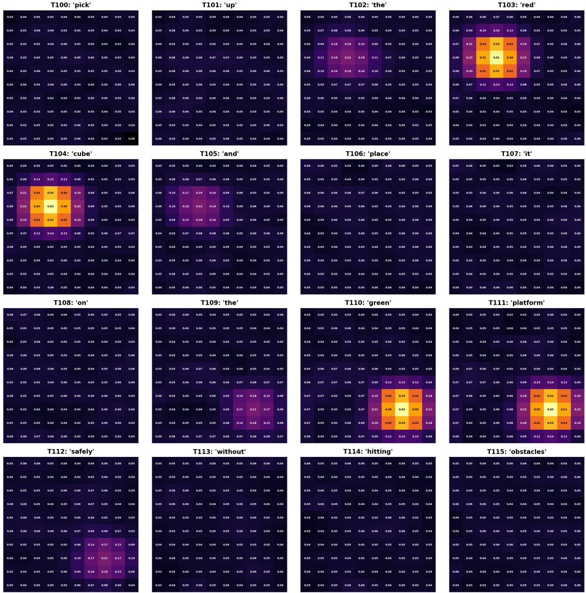
Figure 4: Fine-grained spatial unfold of Layer 20 cross-modal attention. Each grid displays a text token's attention distributed across the 10x10 visual patch space. Values are explicitly annotated and retain their global normalization magnitudes.
