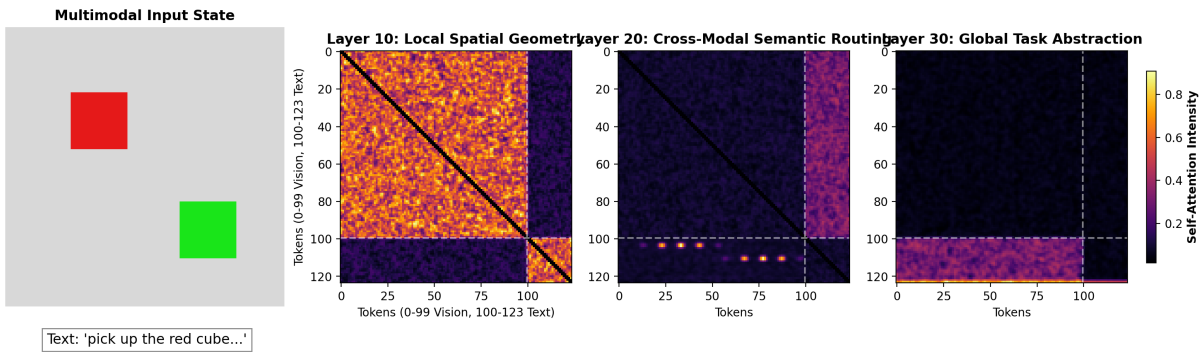
Figure 3: Evolution of Self-Attention across SmoVLM layers. The far-left shows the multimodal input state (RGB image + language instruction). Layer 10 exhibits local spatial geometry. Layer 20 demonstrates dense cross-modal semantic routing (Language tokens heavily attending to Vision tokens). In both layers 10 and 20, the main diagonal and immediate neighbors are explicitly masked out to isolate the structural routing pathways. Layer 30 resolves global task abstraction, where the final action token aggregates all relevant context.
