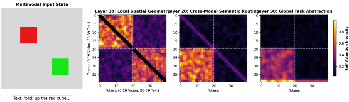
Figure 3: Evolution of Self-Attention across SmoVLM layers. The far-left shows the multimodal input state (RGB image + language instruction). Layer 10 exhibits local spatial geometry (with main diagonal and immediate neighbors explicitly masked out to reveal deeper structural variance). Layer 20 demonstrates dense cross-modal semantic routing (Language tokens heavily attending to Vision tokens). Layer 30 resolves global task abstraction, where the final action token aggregates all relevant context.
