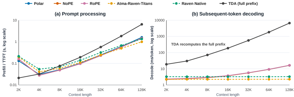
Figure 6: Single-sequence serving on one L40S (logarithmic latency axes). Attention models use cached decoding and Raven uses recurrent state; TDA recomputes the full prefix at each token. Prompt measurements are prefill latency for the cached backends and TTFT for TDA. Backend differences preclude an architecture-only speed comparison.
