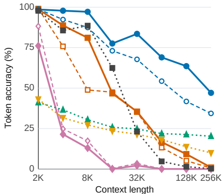
(a) Retrieval
