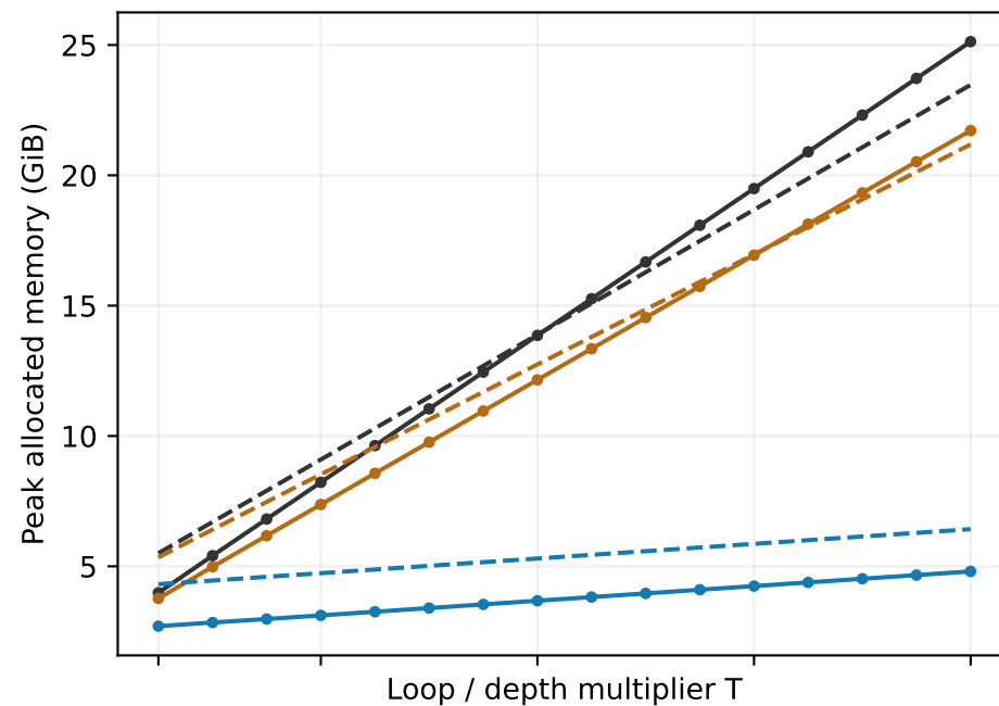
Independent stack
