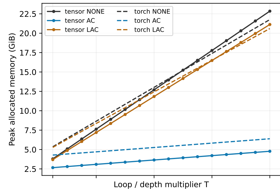
Naive Loop
