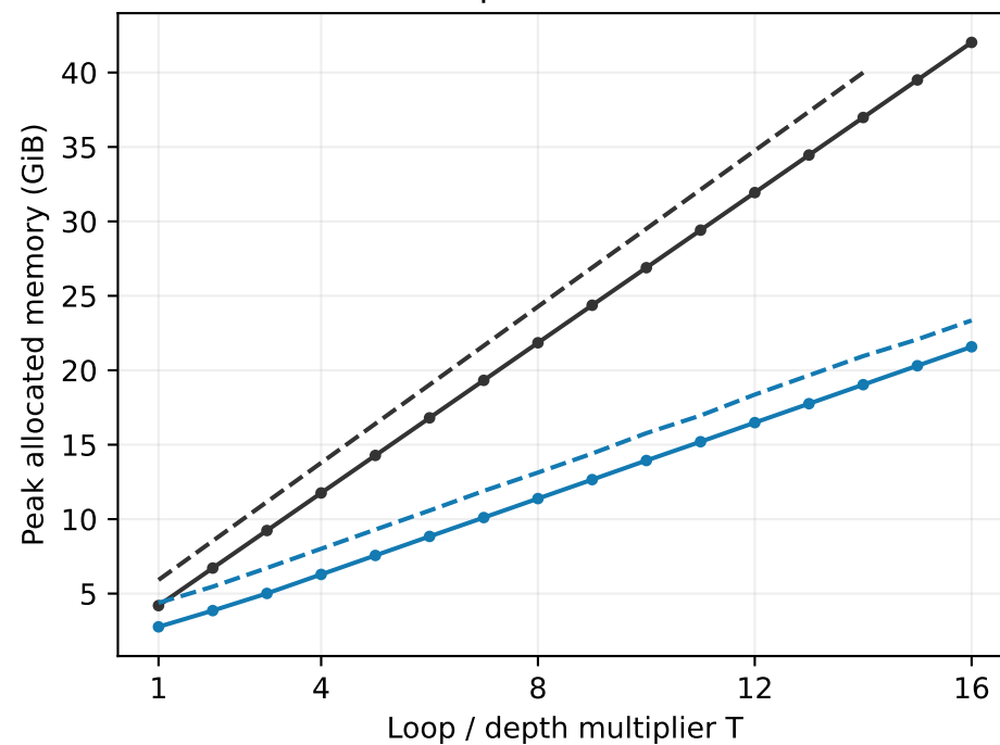
Independent stack
