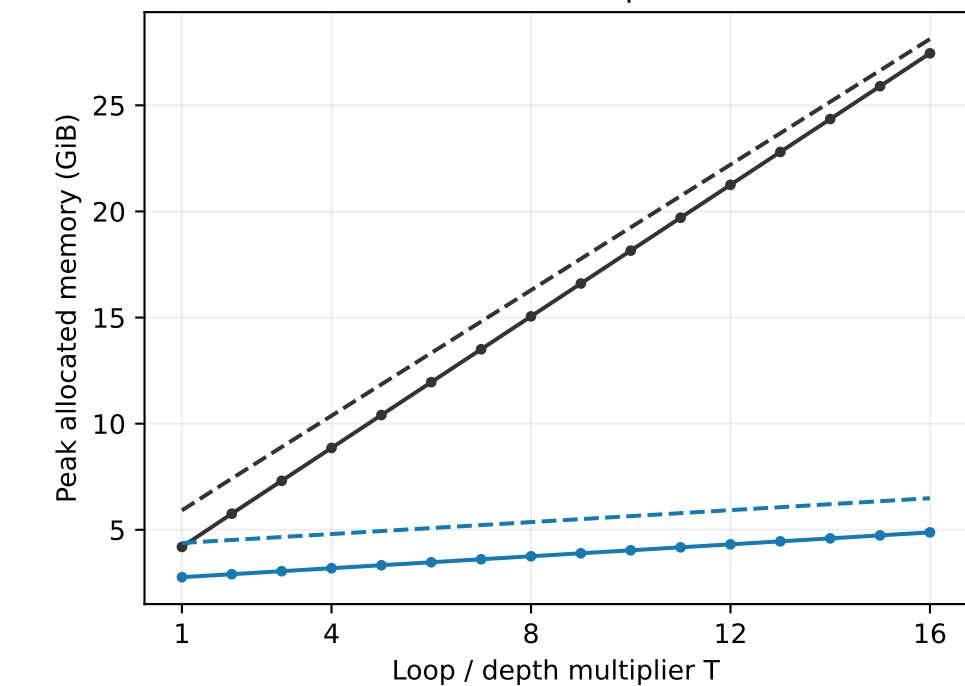
Naive Loop
