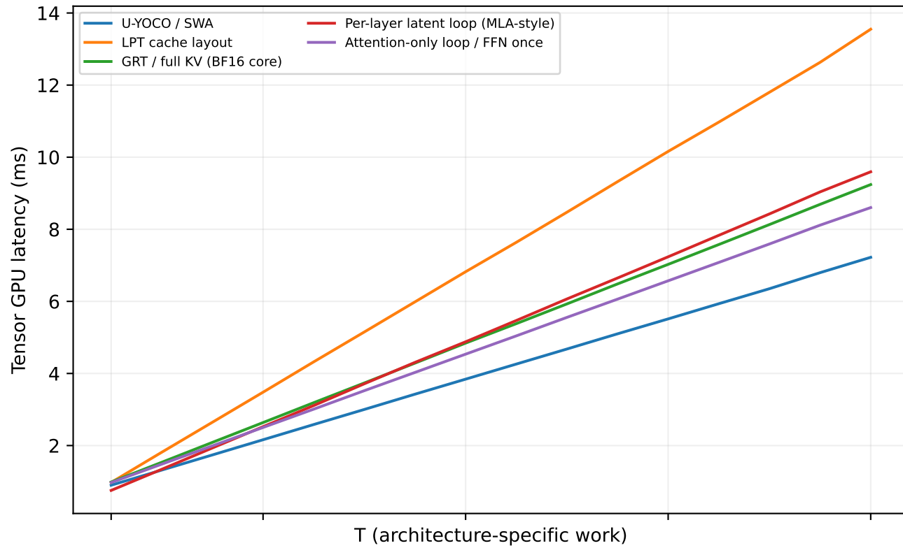
L40S · B4/S1024 · decode graph · architecture kernel adaptations
