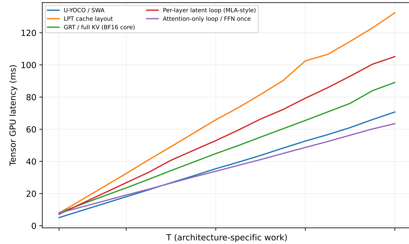
L40S · B4/S1024 · prompt graph · architecture kernel adaptations
