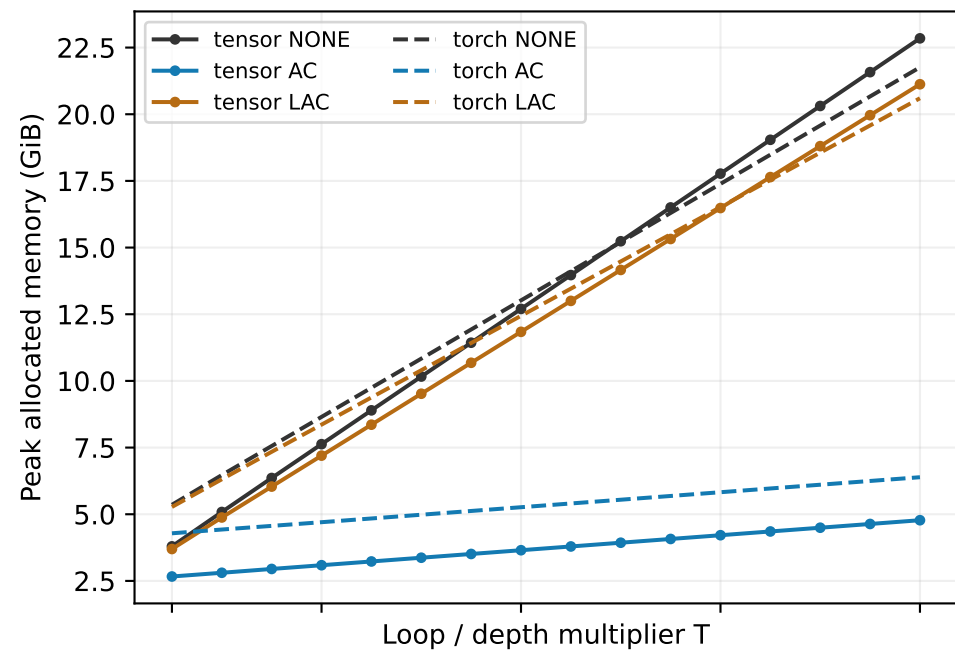
Naive Loop
