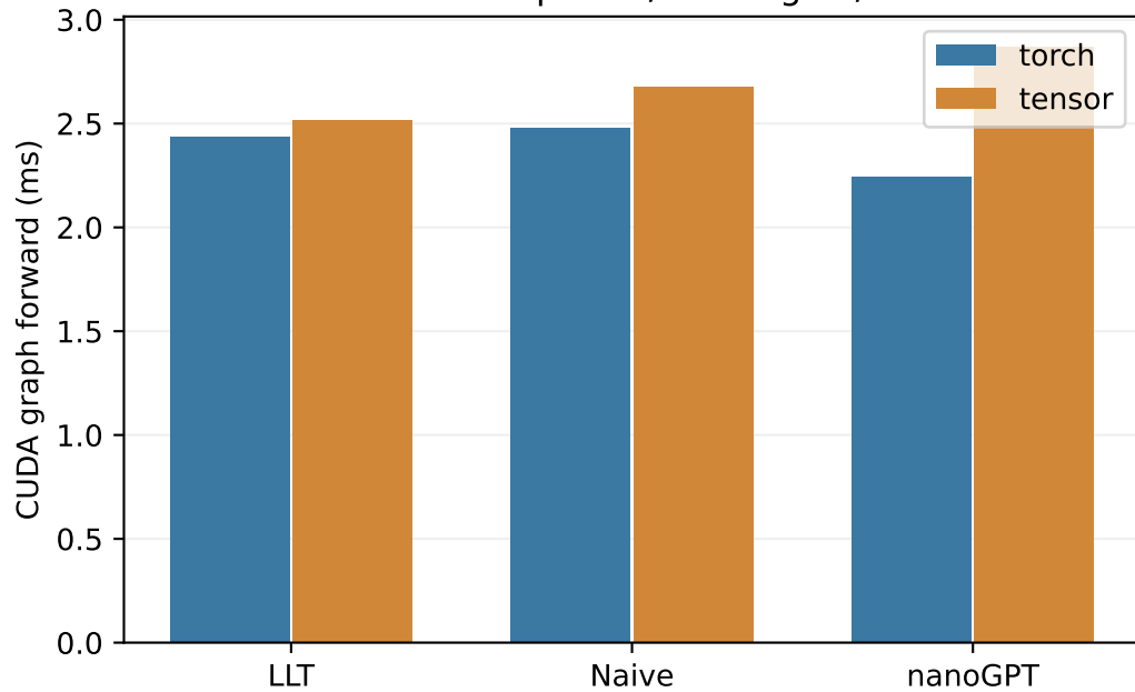
Full causal prefix / last logits / B1
