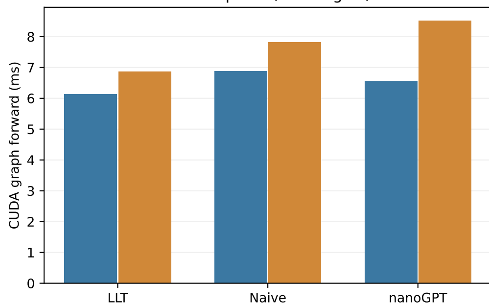
Full causal prefix / last logits / B4
