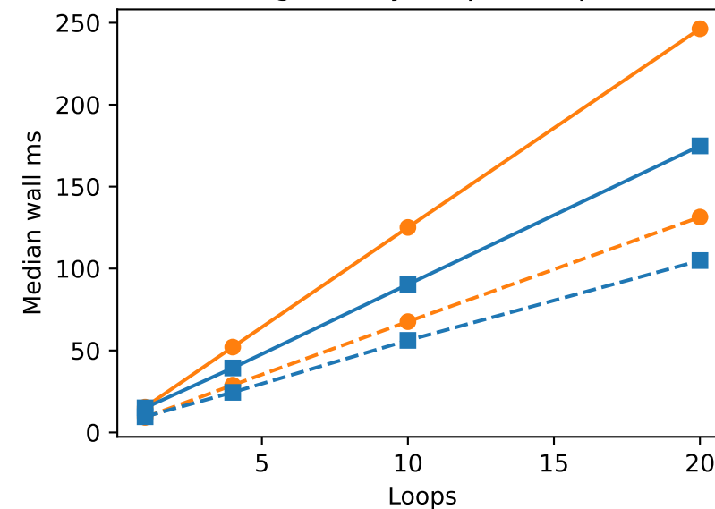
Four-token decode graph latency
