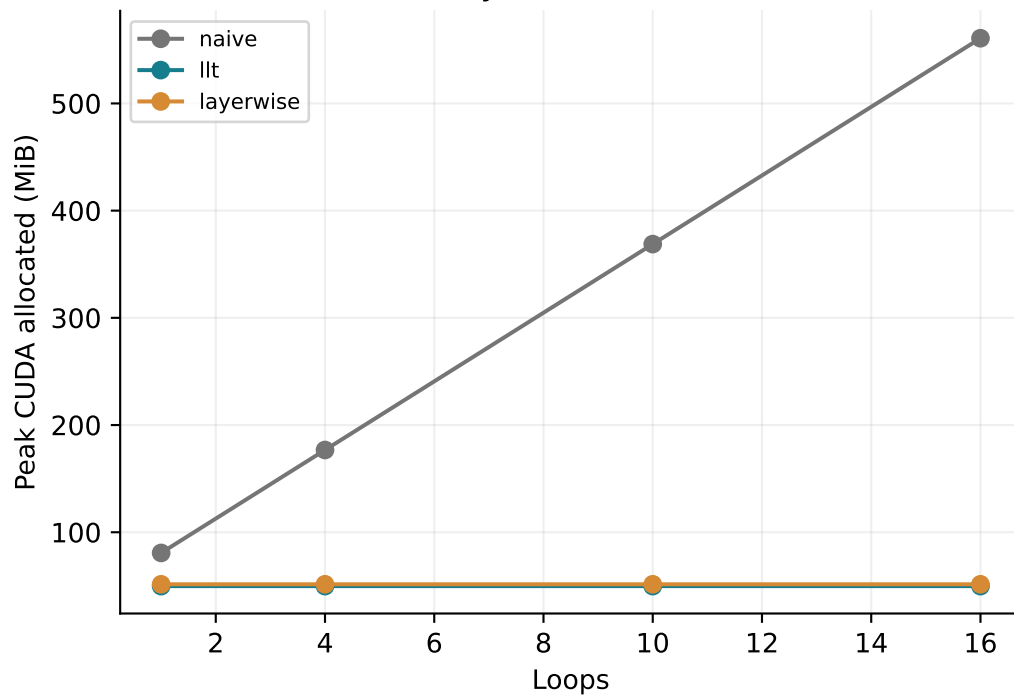
Training memory: W512 / L2 / S1024 / R32
