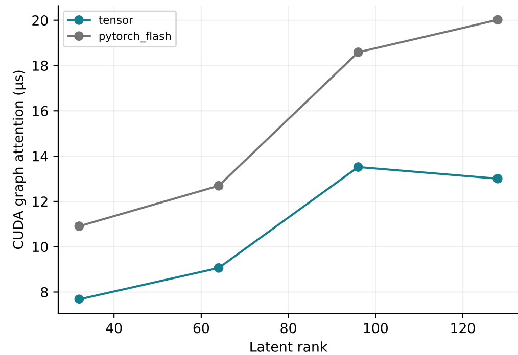
Shared-cache decode kernel: B1 / H8 / S4097
