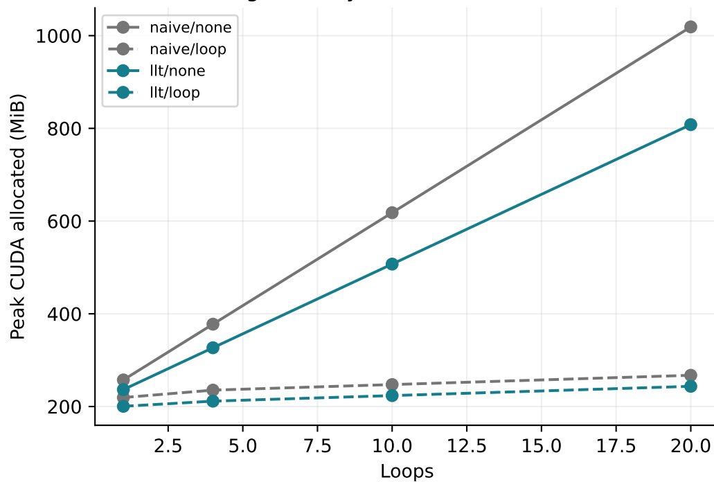
Training memory: W512 / L2 / S1024 / R32
