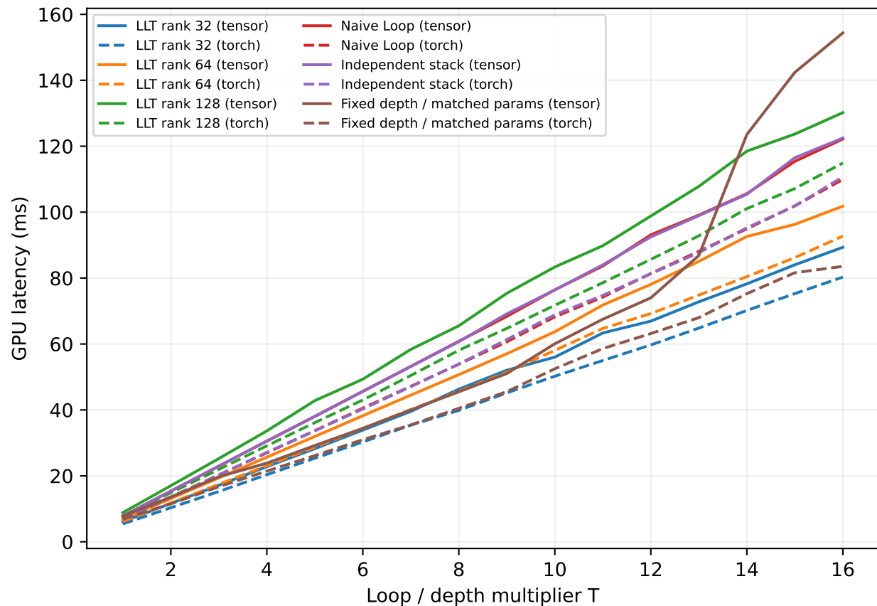
prompt graph · L40S · B4/S1024 · checkpoint policies do not apply
