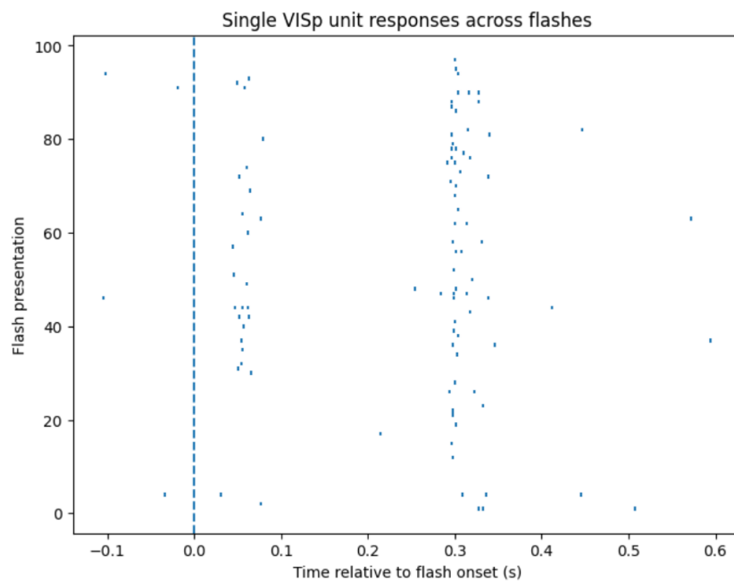
Figure 1: Responses of VISp Unit 8 to flashes. Strong responses observed at around 50 ms and 300 ms.
