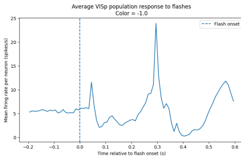
Figure 2: Population Response to Black Flashes
