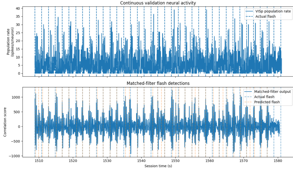
Figure 4: Matched-filter accuracy for the testing set of flashes. An overlap of the orange (predicted flash) and blue (actual flash) means an accurate prediction.
