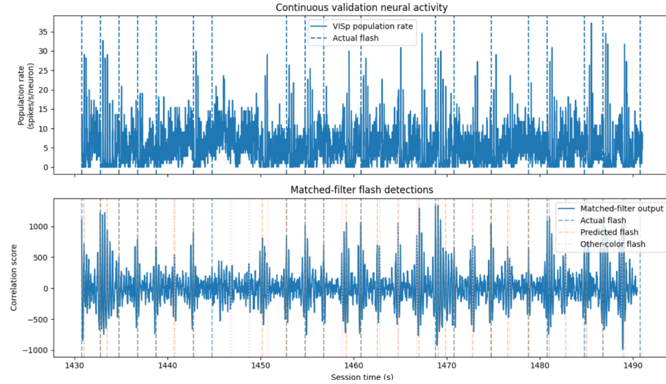
Figure 5: The matched-filter predicted flashes of the other color as well. Overlap of pink (other color flash) and orange (predicted flash) was an indication of this.
