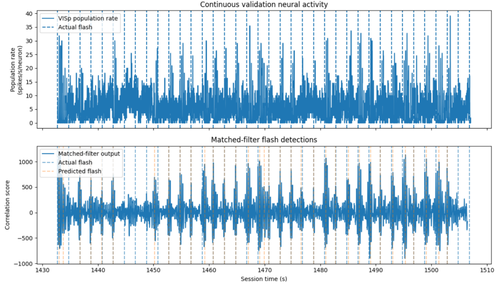
Figure 3: Matched-Filter accuracy for the validation set of flashes. More overlapping orange and blue lines means greater accuracy.
