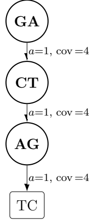
Figure 3: The forest tree-dp builds on (ACGT) 5 : a path, not a star. The discarded edge is parent[GA] = AG (coverage 3), because GA is visited third and by then AG → CT → GA already exists.
