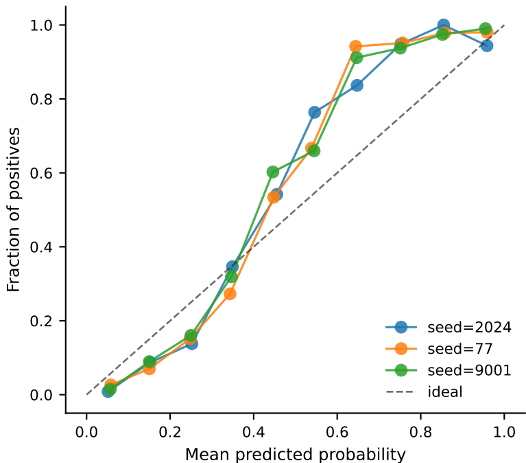
Calibration — random × Random Forest
