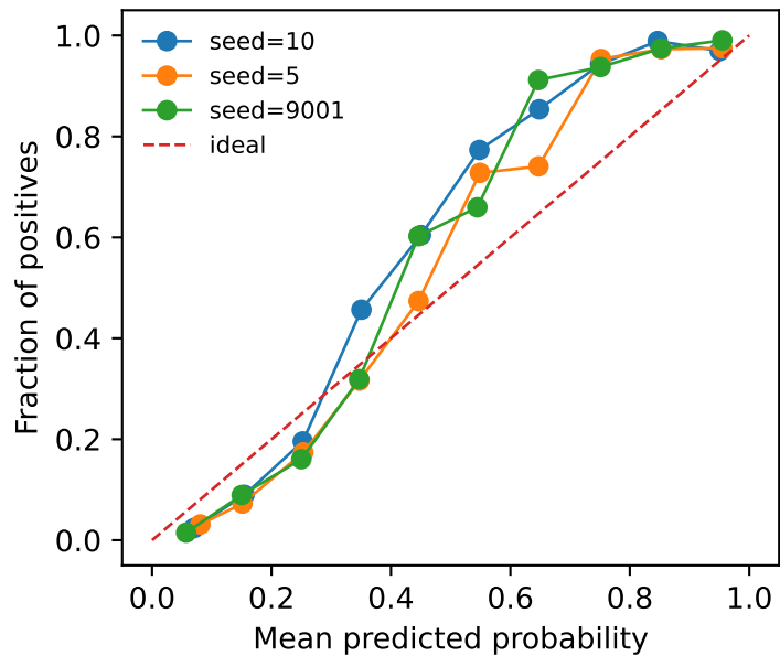
D) Calibration variability — splits
