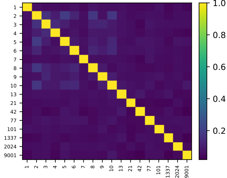
E) Error overlap (Jaccard) — splits
