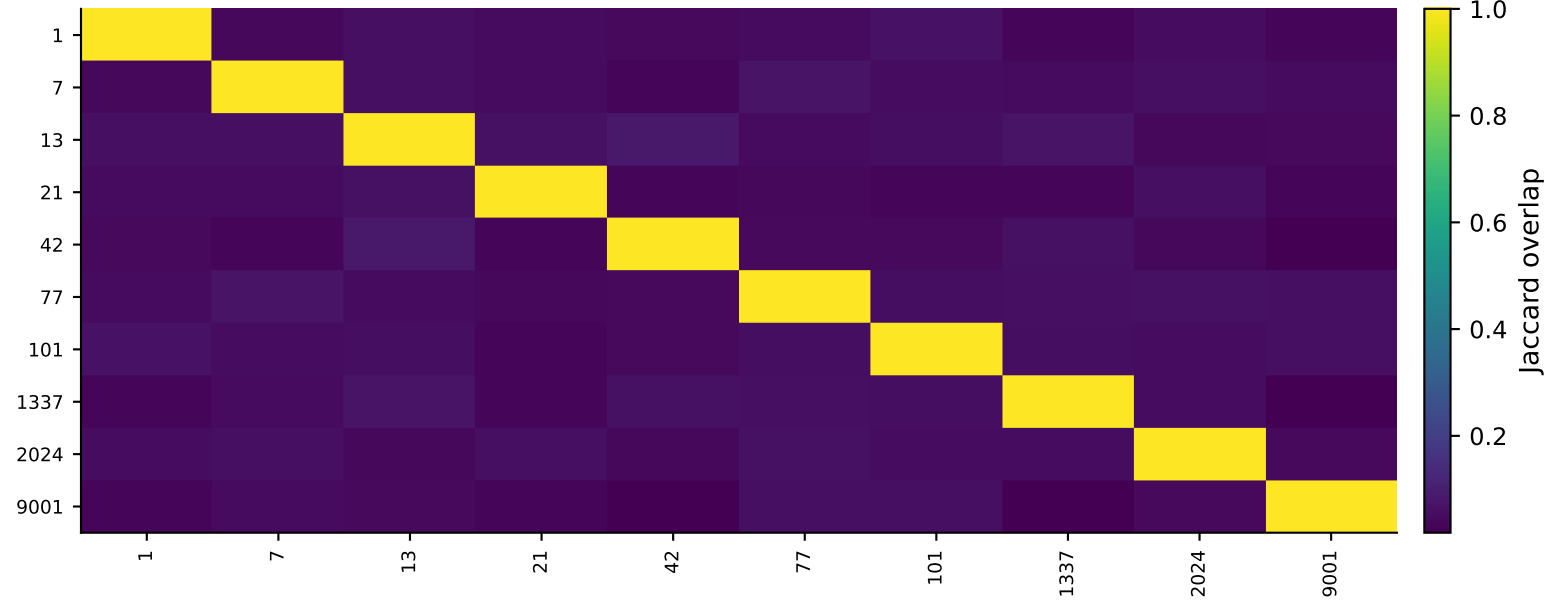
E) Error overlap (Jaccard) — random × random_forest
