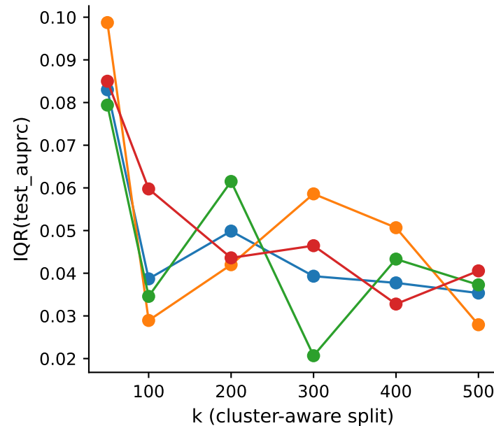
B) Seed fragility vs k (IQR across seeds)
