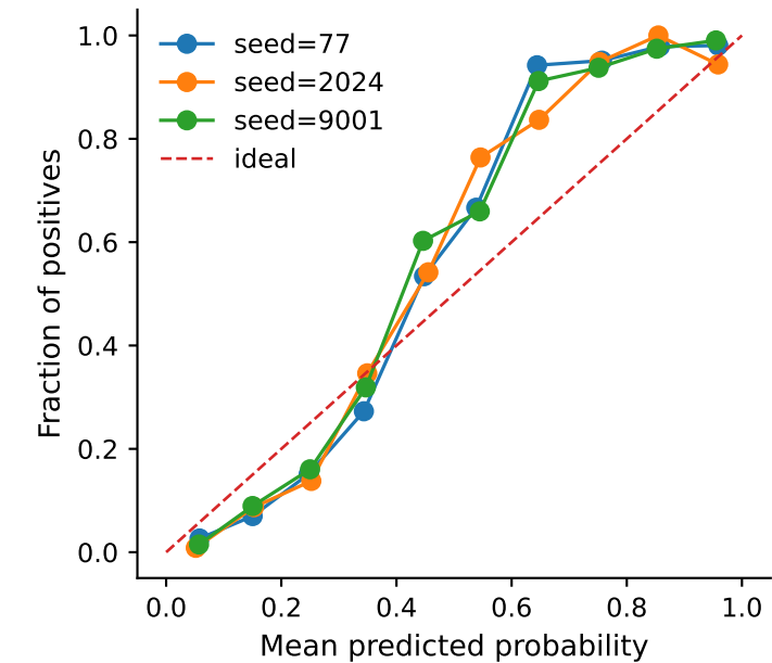
D) Calibration variability — random × random_forest
