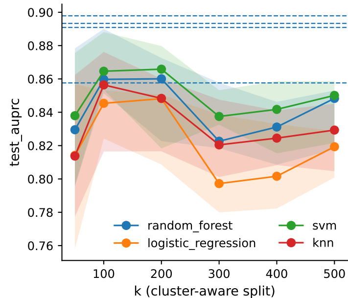
A) Cluster-size effect (median \pm IQR across seeds)
