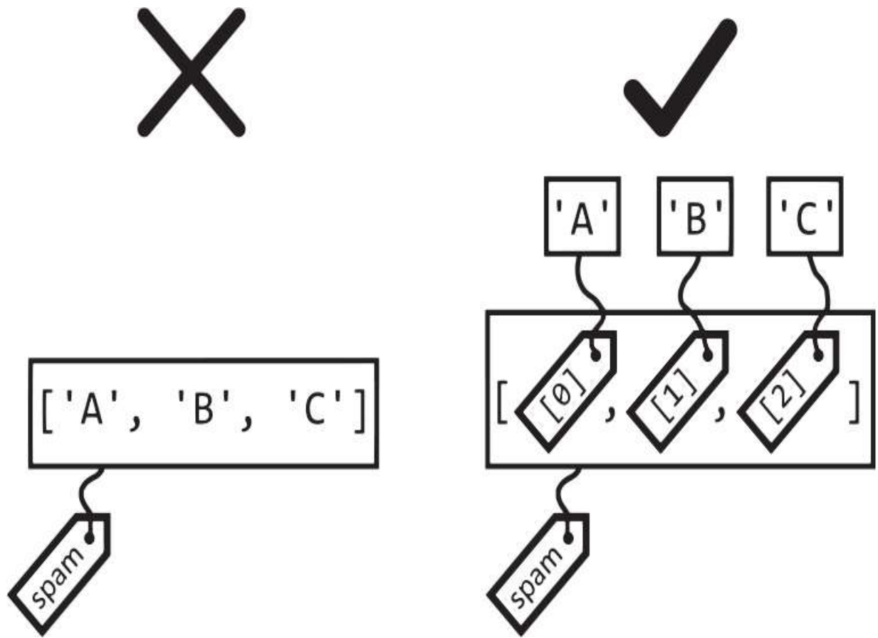
Figure 6-4: Lists don't contain values directly (left); they contain references to values (right).
