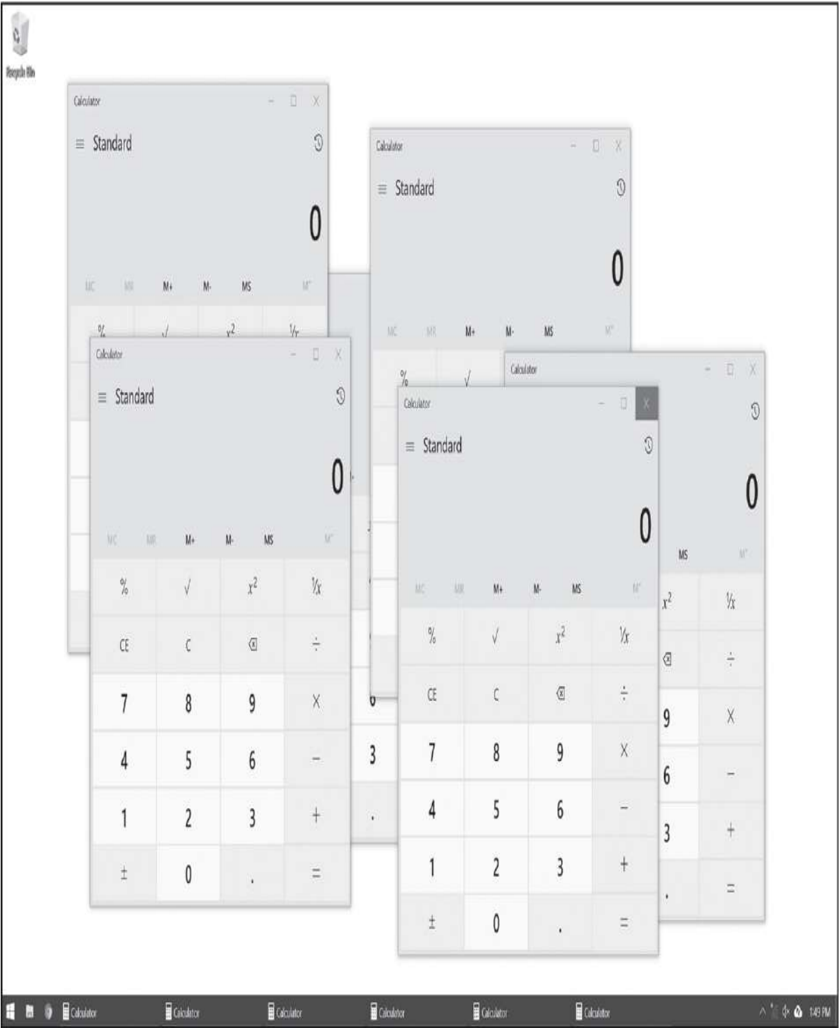
Figure 19-1: Six running processes of the same calculator program
