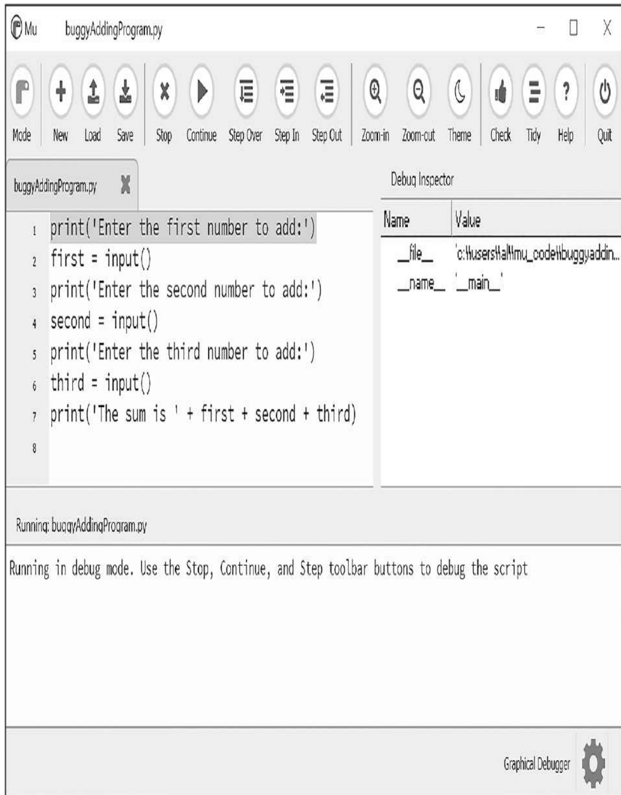
Figure 5-1: Mu running a program under the debugger Description
