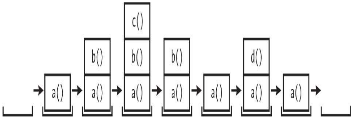
Figure 4-2: The frame objects of the call stack as abcdCallStack.py calls and returns from functions Description
