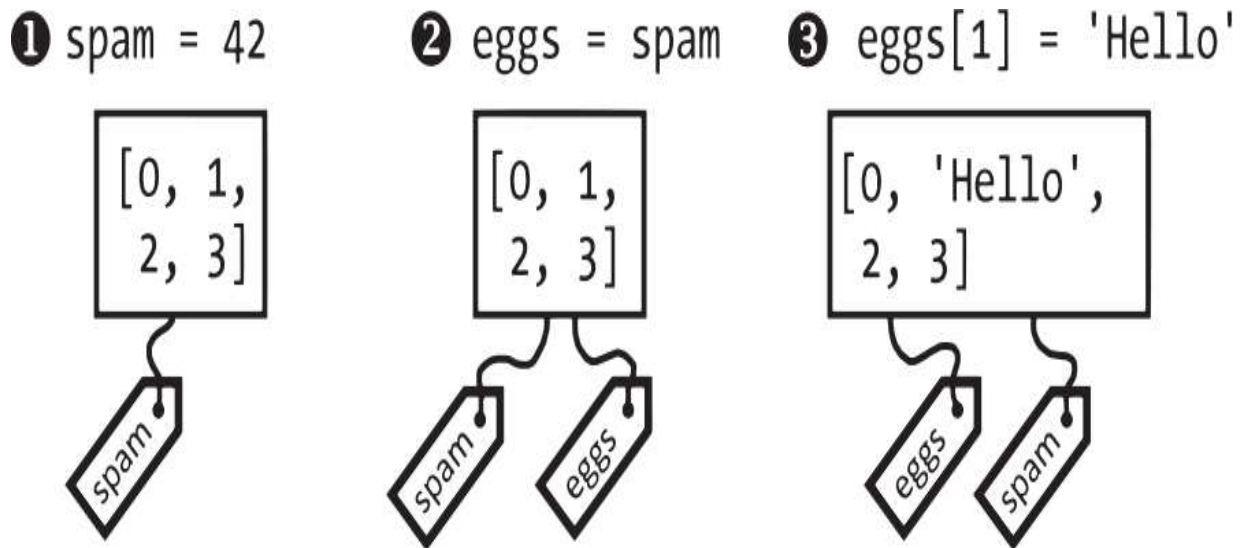
Figure 6-3: Because spam and eggs refer to the same list, changing one changes the other.
