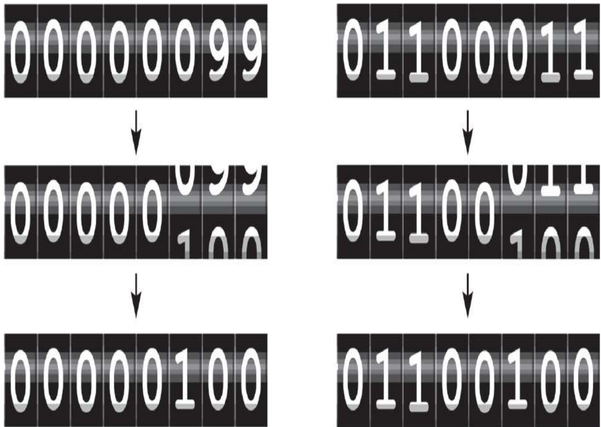
Figure 1-3: A mechanical odometer in decimal (left) and in binary (right)
