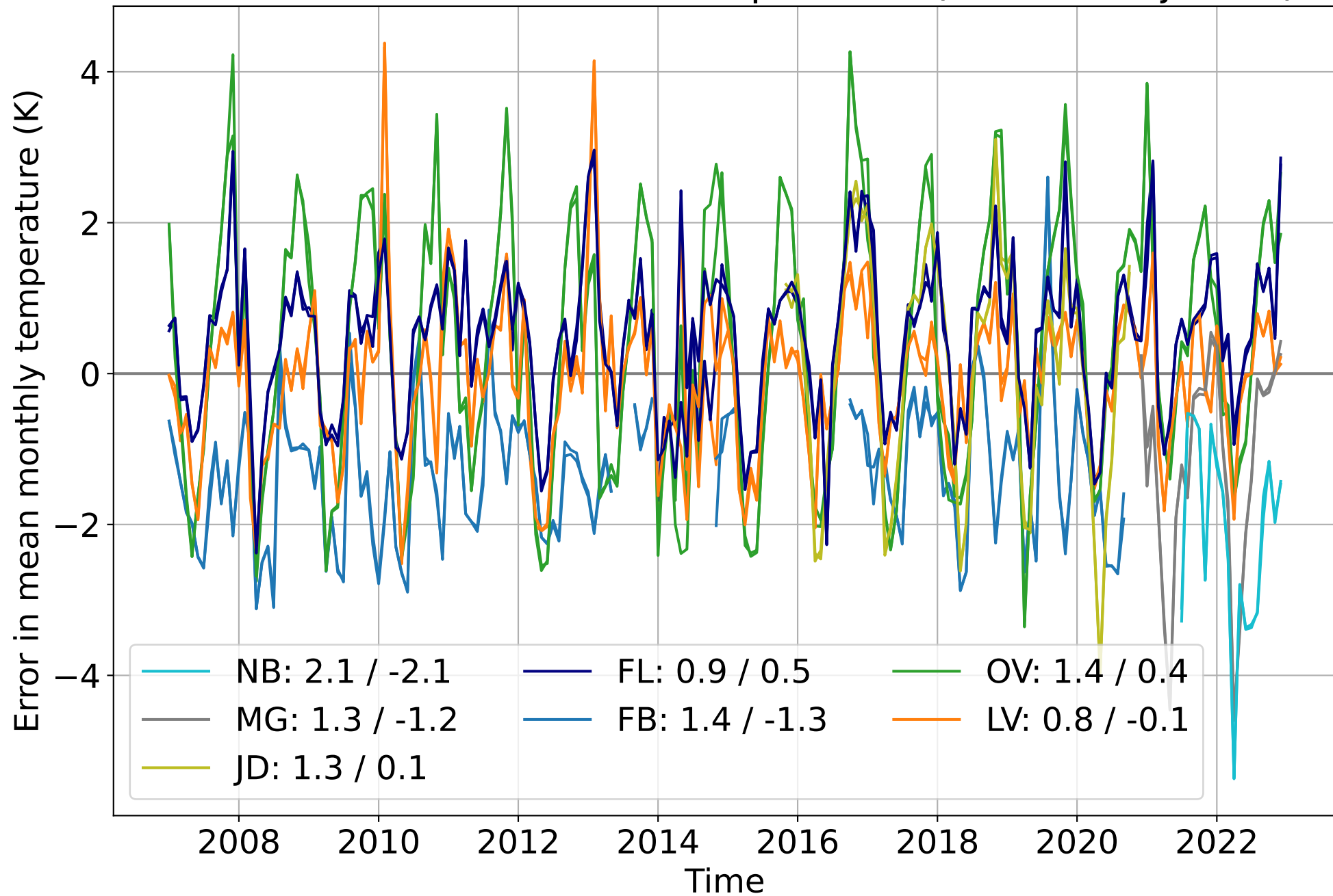
Modelled minus observed temperature (altitude adjusted)
