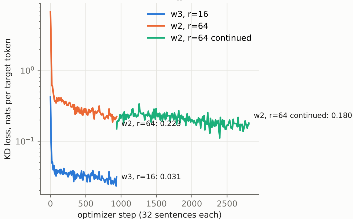
Training loss: KL(fp16 teacher || student)
