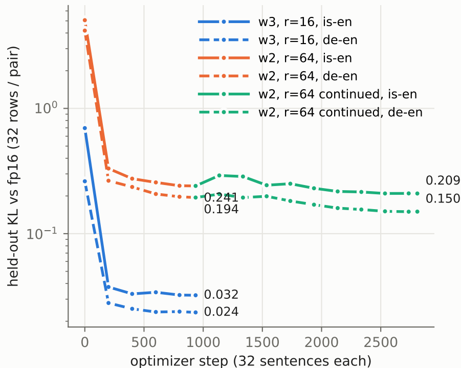
Held-out KL (solid is-en, dashed de-en)
