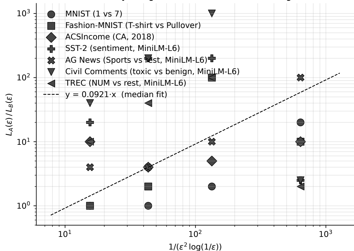
Query-budget ratio vs theoretical scaling
