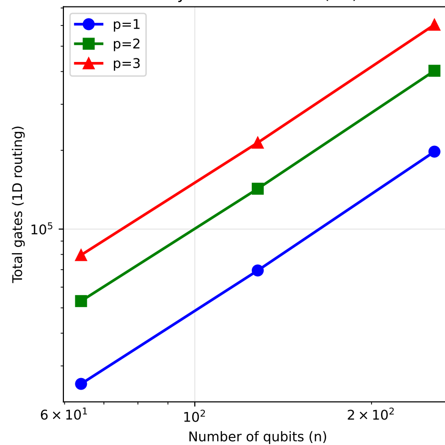
Routing Overhead
