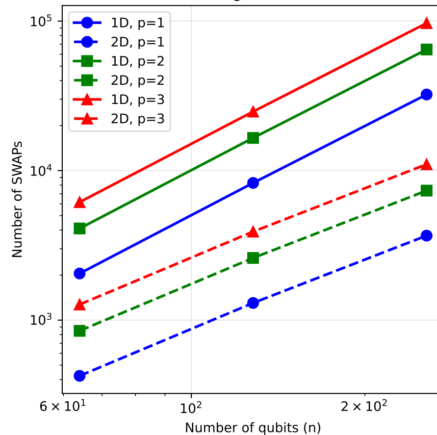
Routing Overhead
